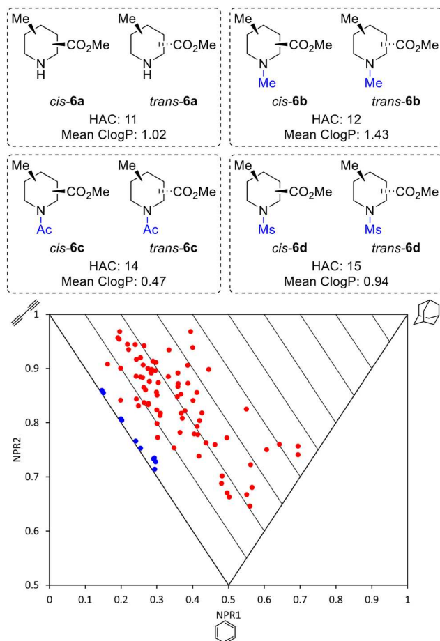
Fig. 2 Molecular properties and PMI plot of the virtual fragment library: cis - and trans -methyl substituted piperidines 6a–d (red dots); pyridines 3 (blue dots) NPR is the normalised principal moment of inertia (see ESI†).
