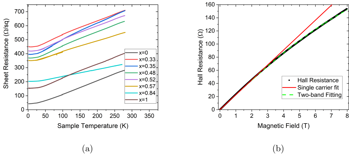
FIG. 3: Summary of transport measurements performed on \text{Bi}_2(\text{Te}_{1-x}\text{Se}_x)_3 samples. a shows the variation in sheet resistance on cooling for the samples studied here. b shows the non-linearity in the Hall trace for the \text{Bi}_2\text{Se}_3 sample, with a linear fit to the low field ( B \leq 1 T) shown in red, and a fit to the full two-band model shown in green.
