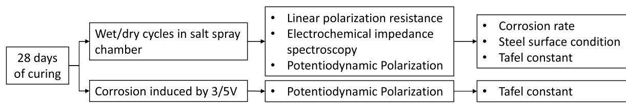
Fig. 4. Schematic representation of corrosion conditions, electrochemical characterization methods and aim of each method.
