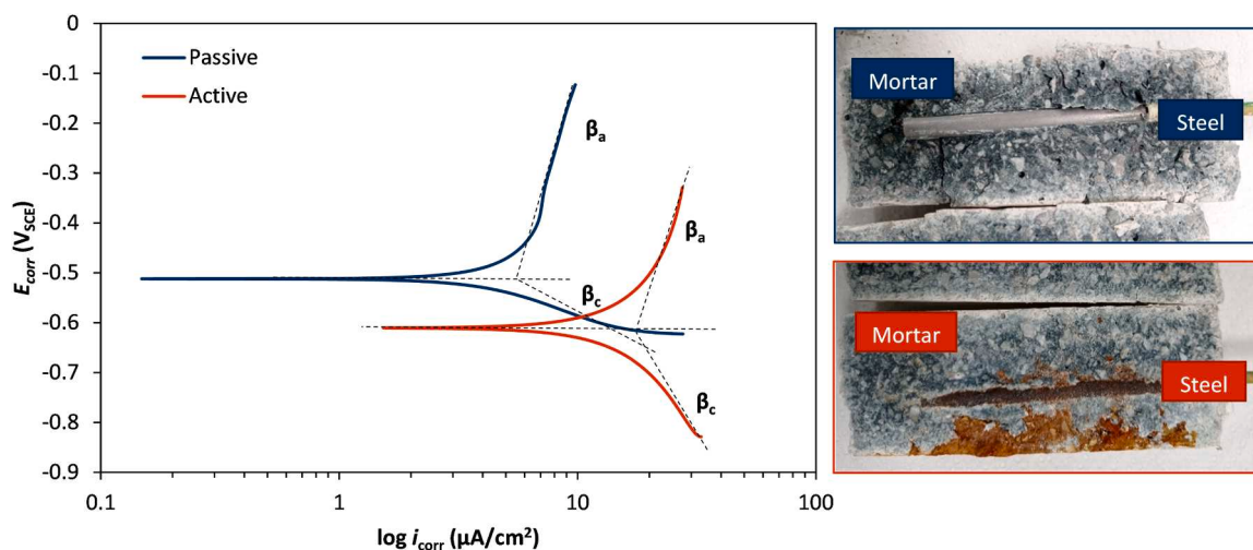
Fig. 15. Example of polarization curves for passive and active SN3 samples, obtained by potentiodynamic polarization E-E_{\text{corr}} = \pm 200 mV, with sweep rates between 2.5 and 10 mV/min, and visual examination of steel surface at the end of measurement.
