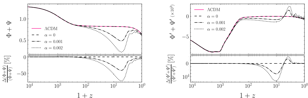
Figure 6. Left panel: (Top) Evolution of the sum of the gravitational potentials as a function of the redshift at k = 0.01 \text{ Mpc}^{-1} for the cases: uncoupled model (dashed line), \alpha = 0.001 (dot-dashed line), \alpha = 0.002 (dotted line), and \Lambda CDM (pink solid line). (Bottom) Relative percentage difference of \Psi + \Phi computed with respect to \Lambda CDM. Right panel: (Top) Evolution of the time derivative of the sum of the gravitational potentials as a function of the redshift (Bottom) Relative percentage difference of \Psi' + \Phi' computed with respect to \Lambda CDM.
