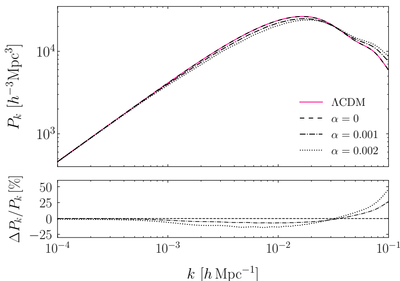
Figure 4. Upper panel: the matter power spectrum as function of k , for the uncoupled case (dashed line), \alpha = 0.001 (dot-dashed line), \alpha = 0.002 (dotted line) and \Lambda\text{CDM} (pink solid line). Lower panel: percentage deviations of the matter power spectrum of the Kinetic model and the uncoupled case from the \Lambda\text{CDM} model.
