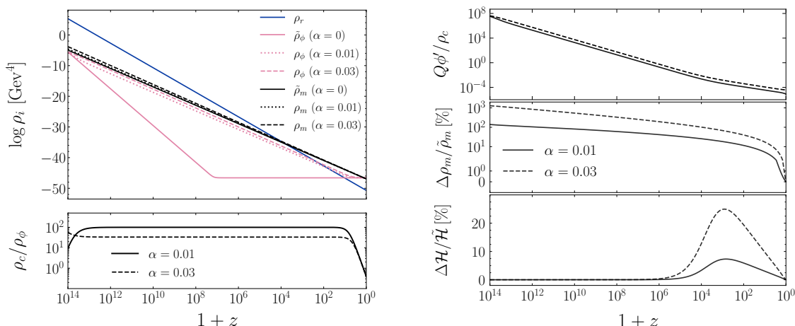
Figure 1. Left upper panel: evolution of the energy densities \rho_i with redshift, 1+z , of the scalar field (pink), matter (black) and radiation (blue) for the uncoupled case (solid line), \alpha = 0.01 (dotted line) and \alpha = 0.03 (dashed line). Left lower panel: ratio of the energy densities of cold dark matter and dark energy, for \alpha = 0.01 (solid line) and \alpha = 0.03 (dashed line). Right panel: differences relative to the uncoupled case, \alpha = 0 , for \alpha = 0.01 (solid line) and \alpha = 0.03 (dashed line), on the quantities (from top to bottom): the coupling strength parameter; the fractional deviation of the energy density of matter, i.e. \Delta\rho_m/\tilde{\rho}_m = \rho_m/\tilde{\rho}_m - 1 , where a tilde denotes variables in the uncoupled scenario, such that \tilde{\rho}_m = \rho_m^0 a^{-3} ; and the fractional deviation of the Hubble rate of expansion.
