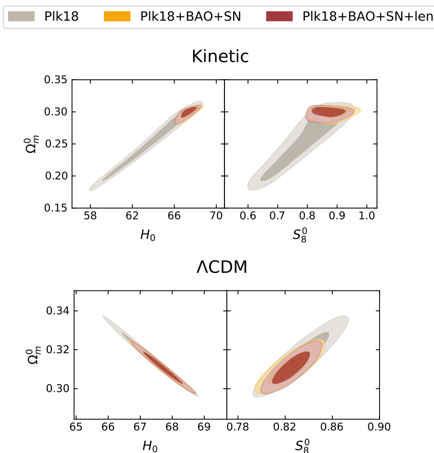
Figure 11. 68% and 95% C.L. 2D contours obtained for the parameters H_0 and \Omega_m^0 (left panels) and S_8^0 and \Omega_m^0 (right panels) in the Kinetic model (upper panels) and \Lambda CDM model (lower panels) for the Planck 2018 data (grey), the Planck 2018, BAO and SN combination (yellow), and their combination with CMB lensing (red).
