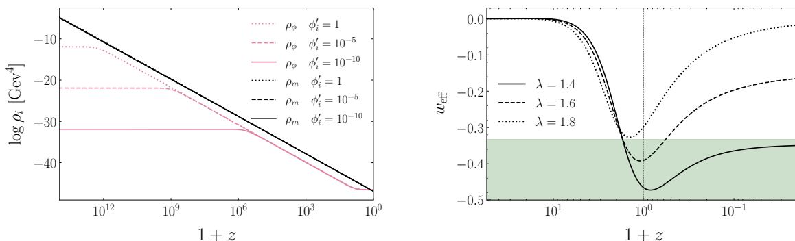
Figure 3. Left Panel: evolution of the energy densities of matter (black) and scalar field (pink) for different ICs for the field’s velocity, \phi'_i , with fixed \alpha = 0.03 and \lambda = 0.2 . Right Panel: effective equation of state, w_{\text{eff}} , for different values of \lambda , namely \lambda = 1.4 (solid line), \lambda = 1.6 (dashed line) and \lambda = 1.8 (dotted line), with fixed \alpha = 0.03 . The shaded green area corresponds to the region where the Universe features accelerated expansion, i.e. w_{\text{eff}} < -1/3 .
