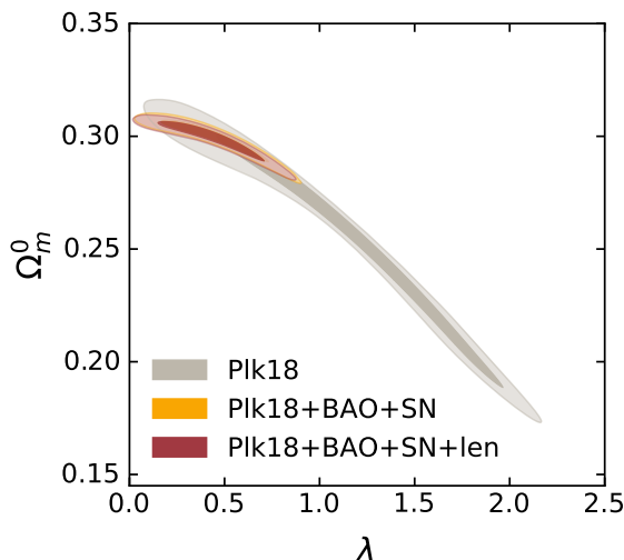
Figure 12. 68% and 95% C.L. 2D contours obtained for the parameters \lambda and \Omega_m^0 for the Kinetic model considering the Planck 2018 data (grey), the Planck 2018, BAO and SN combination (yellow), and their combination with CMB lensing (red).
