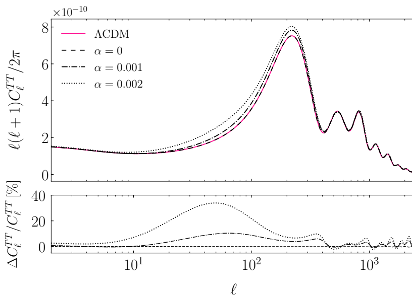
Figure 8. Upper panel: TT power spectrum as function of the angular scale \ell , for the uncoupled case (dashed line), \alpha = 0.001 (dot-dashed line), \alpha = 0.002 (dotted line) and \Lambda CDM (pink solid line) for reference. Lower panel: percentage deviations of the TT power spectra for the coupled and uncoupled cases with respect to \Lambda CDM.
