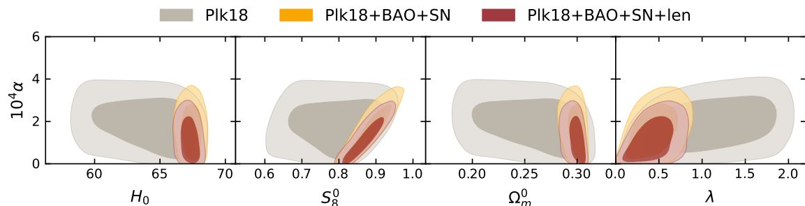
Figure 9. 68% and 95% C.L. contours obtained in the Kinetic model under consideration for the Planck 2018 data (grey), the Planck 2018, BAO and SN combination (yellow), and their combination with CMB lensing (red).
