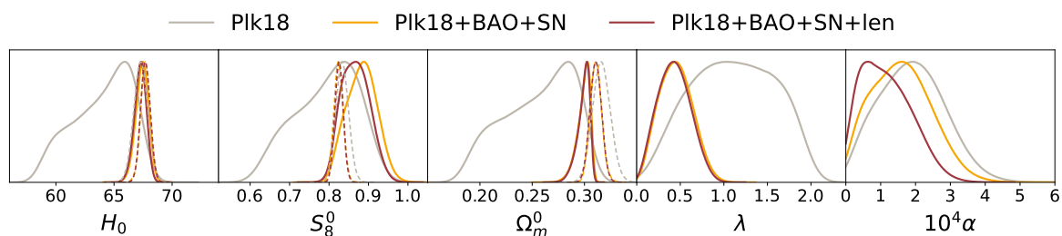
Figure 10. Comparison between the \Lambda CDM (dashed lines) and Kinetic model (solid lines) marginalised likelihood of the cosmological parameters for the Planck 2018 data (grey), the Planck 2018, BAO and SN combination (yellow) and their combination with CMB lensing (red).
