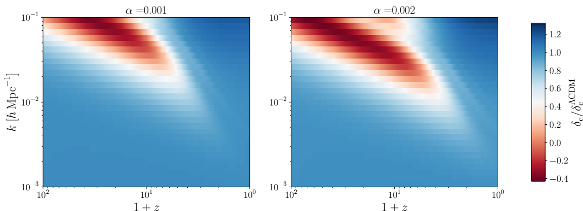
Figure 5. Evolution of the density contrast of cold dark matter for the Kinetic model relative to the \Lambda CDM case, that is \delta_c/\delta_c^{\Lambda\text{CDM}} , as a function of the Fourier scale k and the redshift z for \alpha = 0.001 and \alpha = 0.002 .
