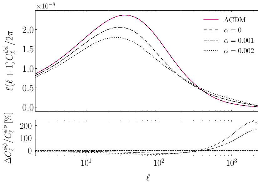
Figure 7. Upper panel: lensing angular power spectra for \Lambda CDM (solid pink line), \alpha = 0.001 (dot-dashed line), \alpha = 0.002 (dotted line) and the uncoupled case (dashed line). Lower panel: relative difference between the lensing power spectra of each model and that of \Lambda CDM.
