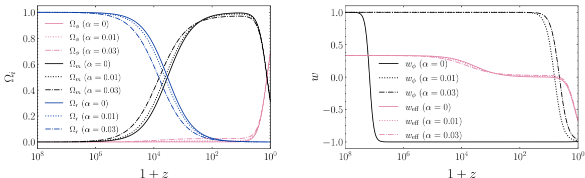
Figure 2. Left panel: evolution of the relative energy densities \Omega_i with redshift, 1+z , of the scalar field (pink), matter (black) and radiation (blue). Right panel: equation of state parameters, w_{\text{eff}} (pink) and w_\phi (black), along redshift. In accordance with figure 1, we present the uncoupled case (solid line), \alpha = 0.01 (dotted line) and \alpha = 0.03 (dot-dashed line).
