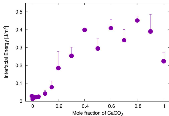
Fig. 2. Interfacial energy of calcite (10.4) surface with h -ACC for 0 < x_{\text{CaCO}_3} < 1 . Error bar shown covers the range between the minimum value calculated for the three configurations (purple circle) and the maximum value for the three configurations (top of the error bar). (For interpretation of the references to colour in this figure legend, the reader is referred to the web version of this article.)
