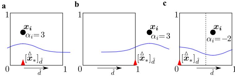
Fig. 2 Examples of three configurations of the training point's location ( [x_i]_{\hat{d}} ) and value ( \alpha_i ), to illustrate where \alpha_i k(x_i, \hat{x}_*) is maximised. One can easily see the equivalent locations which minimise the expression. Here we have chosen a = 0 and b = 1 . a If 0 \leq [x_i]_{\hat{d}} \leq 1 and \alpha_i \geq 0 , \alpha_i k(x_i, \hat{x}_*) is maximised if [\hat{x}_*]_{\hat{d}} = [x_i]_{\hat{d}} . b If [x_i]_{\hat{d}} \geq 1 and \alpha_i \geq 0 , \alpha_i k(x_i, \hat{x}_*) is maximised if [\hat{x}_*]_{\hat{d}} = 1 . c If [x_i]_{\hat{d}} \geq \frac{1}{2} and \alpha_i \leq 0 , \alpha_i k(x_i, \hat{x}_*) is maximised if [\hat{x}_*]_{\hat{d}} = 0
