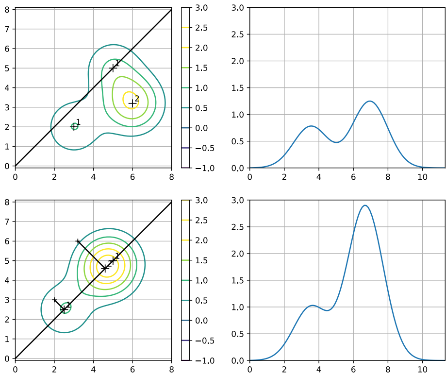
Fig. 3 Upper left, contour plot of the sum of three, two-dimensional EQs. Upper right, the values of the sum along the diagonal, one-dimensional line. Lower left, the effect on the contour plot if the three points are placed on the diagonal line to illustrate the effect of a principle component approximation. Lower right, the sum along the diagonal line. Note that this new function is never less than the function for when the EQ points are spaced in the full two-dimensional domain
