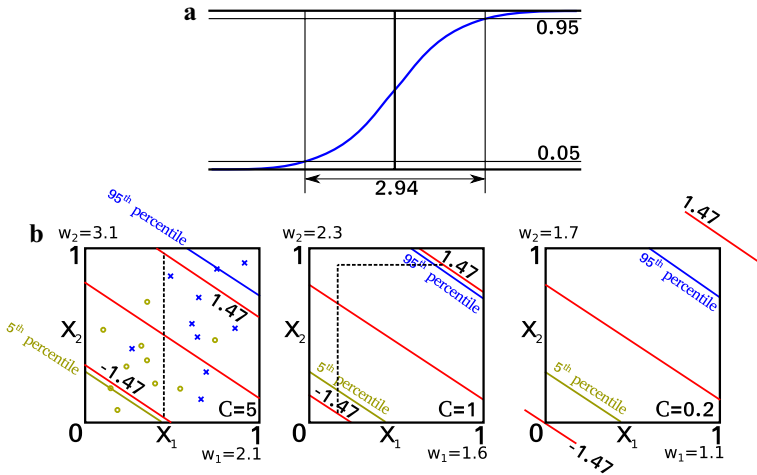
Fig. 1 2d example using logistic regression. a The logistic function, to move from 5% to 95% confidence requires a change of 2.94 in the latent function, w_0 + x_1 w_1 + x_2 w_2 . b Left plot , least regularisation: moving between thresholds is possible by changing just one input, x_2 (as |w_2| > 2.94 ), see dashed line. Middle plot : greater regularisation. It is only possible to move between the thresholds by altering both inputs (as |w_1| < 2.94 & |w_2| < 2.94 ). Right plot : even more regularisation. It becomes impossible to move between the two thresholds (i.e. when |w_1| + |w_2| < 2.94 ) even changing all inputs! We suggest rather than use fixed values for these thresholds one should use the values of the 5th and 95th percentile training points (orange and blue lines) to assess the robustness of a classifier. C is inverse L_2 regularisation (Color figure online)
