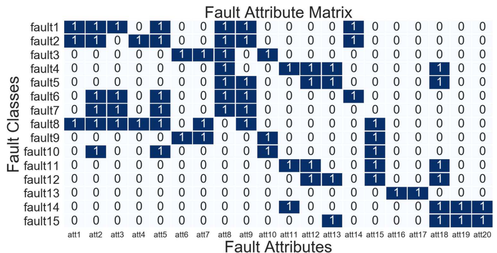
Fig. 8 Fault attribute matrix A [3]
