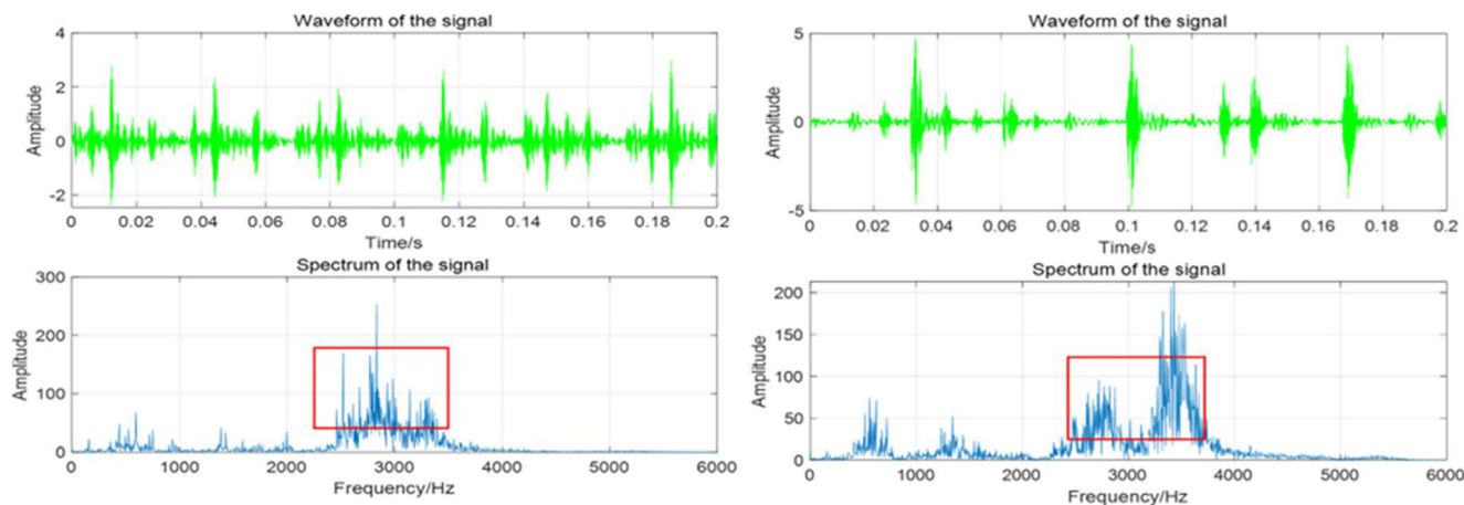
Fig. 6 Time-domain signal and frequency-domain signal of fault 7 and fault 9 in 3hp
