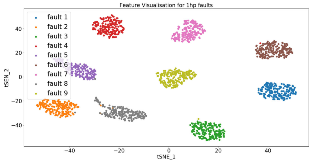
Fig. 4 The t-SNE results of the output features of the FC layer for the case of working load 1 hp. The horizontal and vertical coordinates represent the first two principal components extracted from t-SNE, respectively
