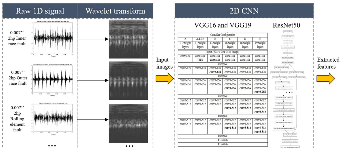
Fig. 7 Procedure of 2D feature extraction
