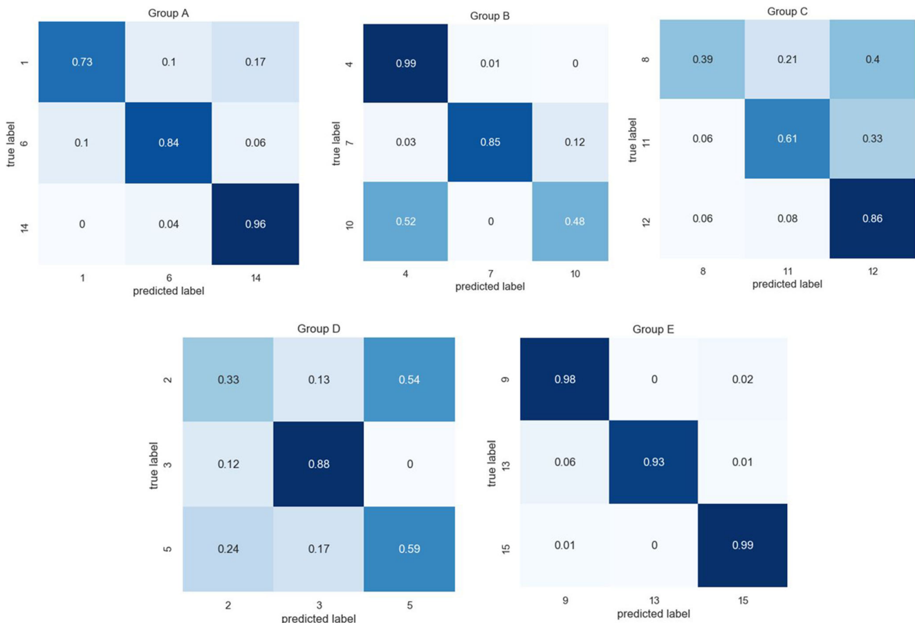
Fig. 9 Confusion matrices of the results of unseen faults
