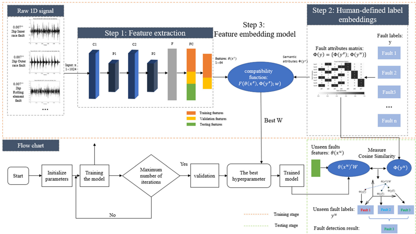
Fig. 1 The structure of the proposed method
