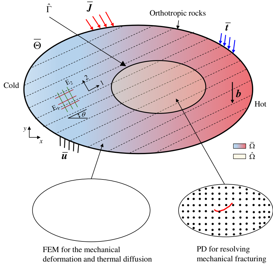
Fig 1 Schematics of the superposition-based coupling of PD and FEM approach for thermal fracturing analysis in orthotropic rocks
