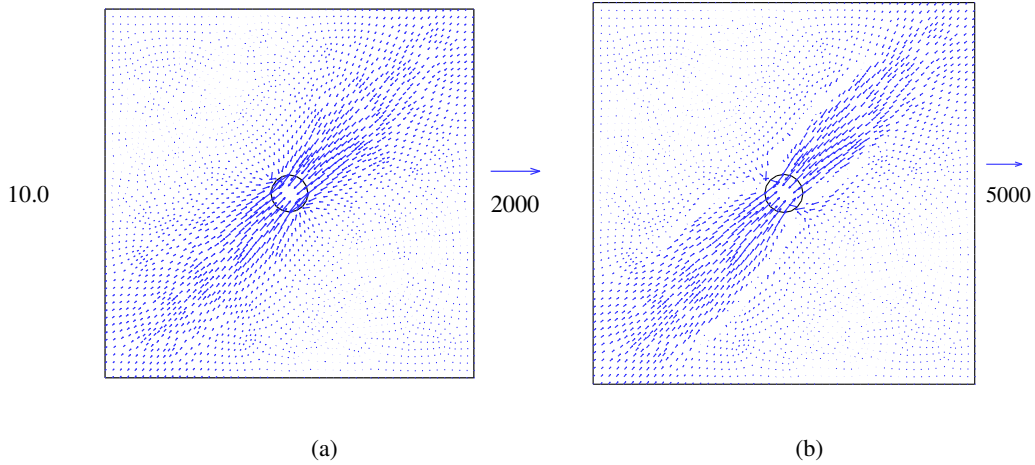
Fig. 16 Thermal fracturing in an orthotropic rock specimen under high surrounding temperature with different ratios of k_1/k_2 : (a) heat flux directions at time t = 2.0 \times 10^5 s (prior to the crack initiation); (b) heat flux directions at the steady state
