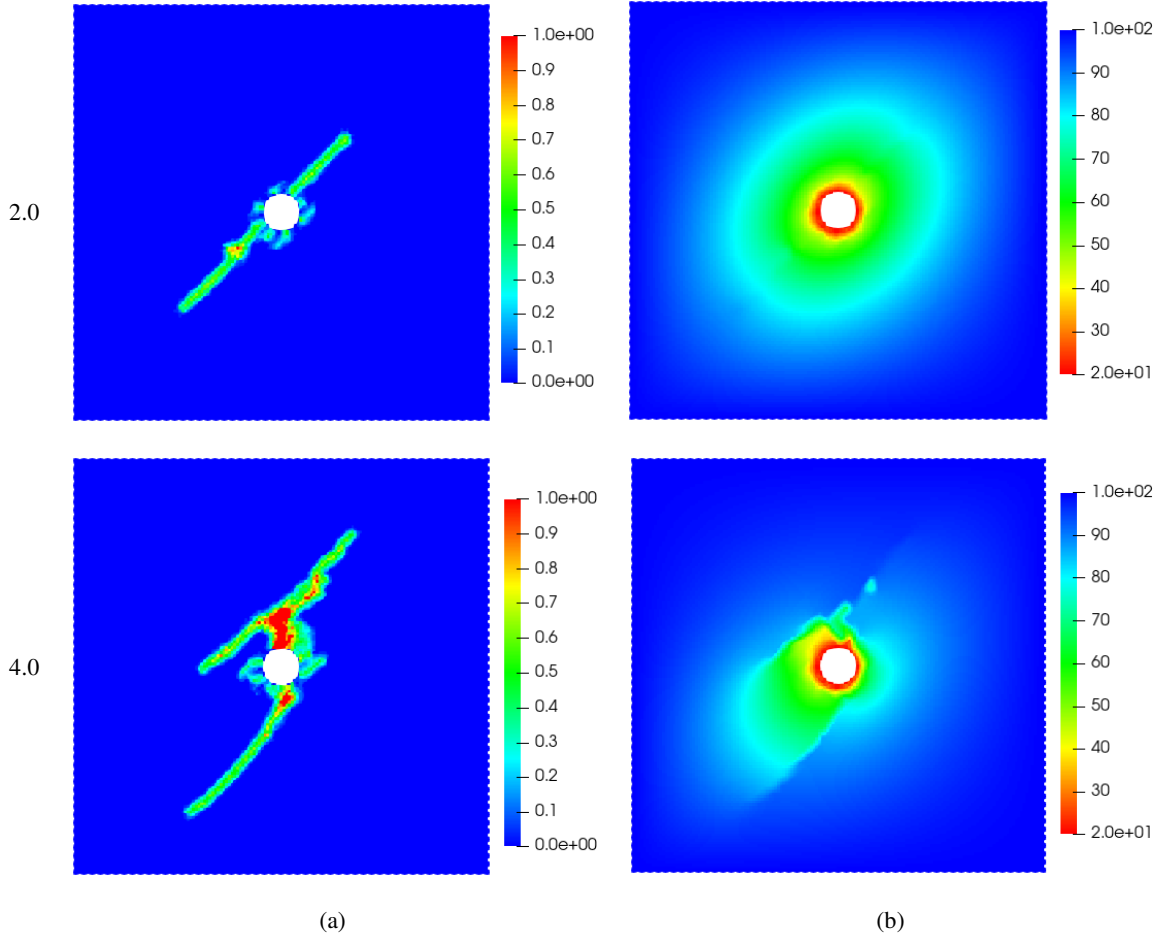
Fig .13 Thermal fracturing in an orthotropic rock specimen under high surrounding temperature with different ratios of E_1/E_2 : (a) crack paths; (b) temperature distribution (units: ^{\circ}\text{C} )
