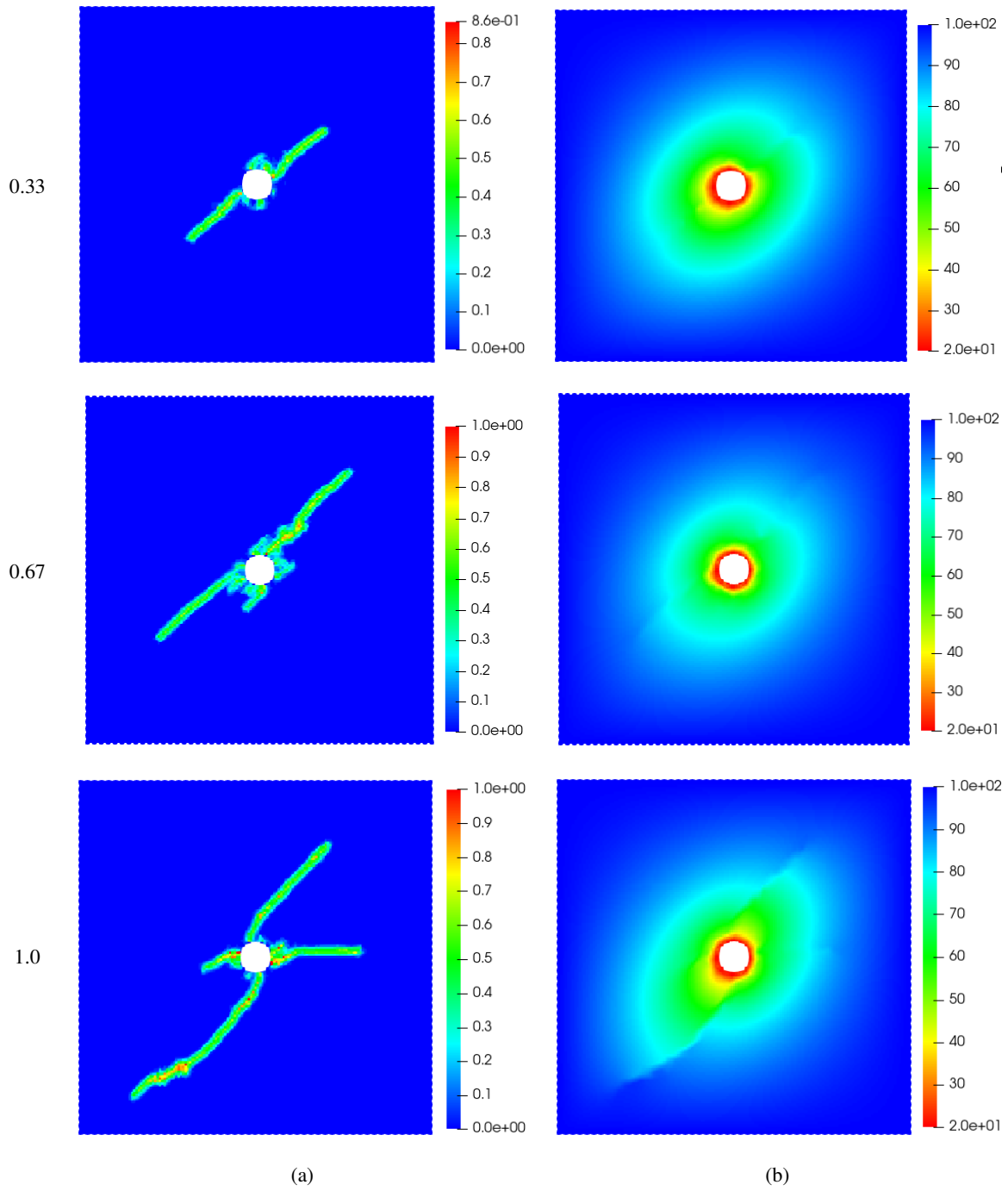
Fig. 17 Thermal fracturing in an orthotropic rock specimen under high surrounding temperature with different ratios of a_1/a_2 : (a) crack paths; (b) temperature distribution (units: ^{\circ}\text{C} )
