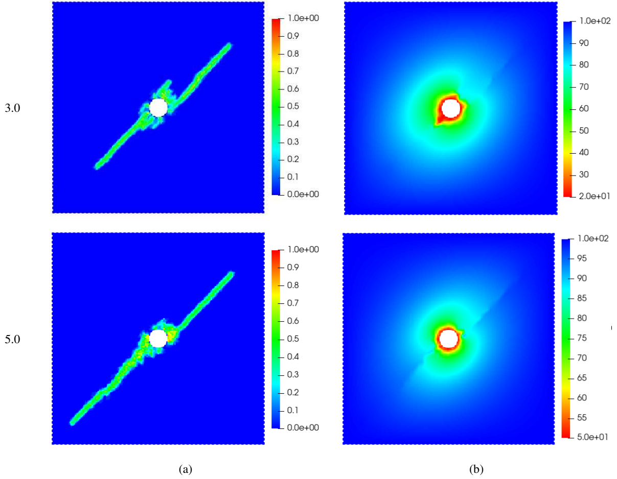
Fig. 14 Thermal fracturing in an orthotropic rock specimen under high surrounding temperature with different ratios of G_1/G_2 : (a) crack paths; (b) temperature distribution (units: ^{\circ}\text{C} )
