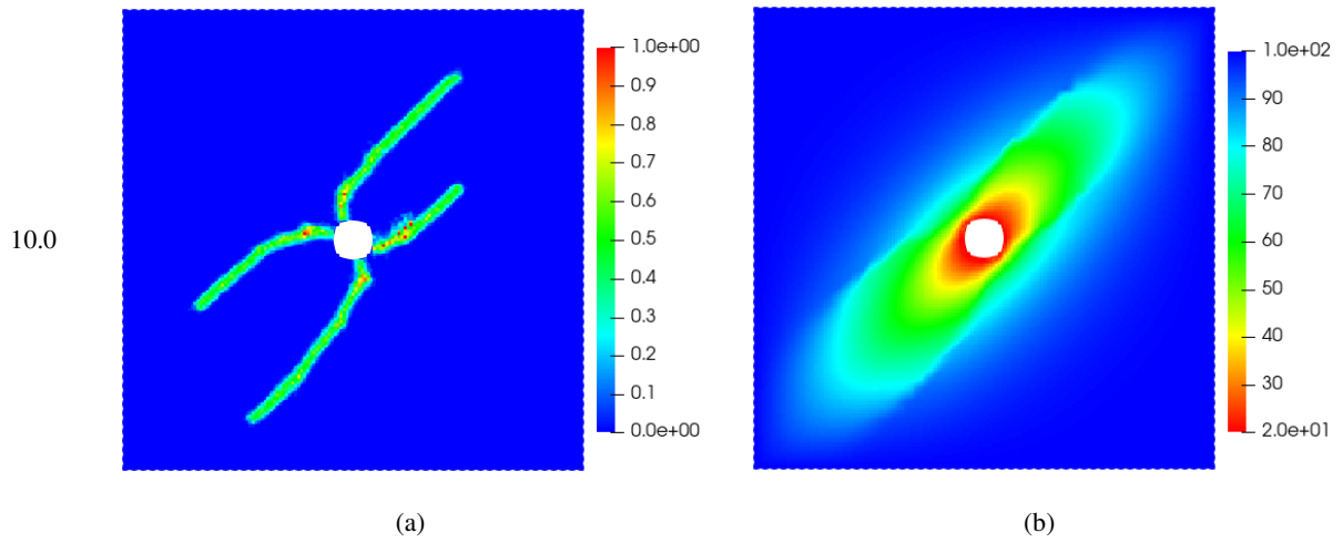
Fig. 15 Thermal fracturing in an orthotropic rock specimen under high surrounding temperature with different ratios of k_1/k_2 : (a) crack paths; (b) temperature distribution (units: °C)
