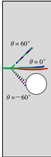
Fig. 7 Crack trajectories obtained by different models: XFEM (Bayat and Nazari, 2021; red lines), extended four-node consecutive-interpolation element method (Nguyen et al., 2019; blue lines) and the proposed method (green lines)
