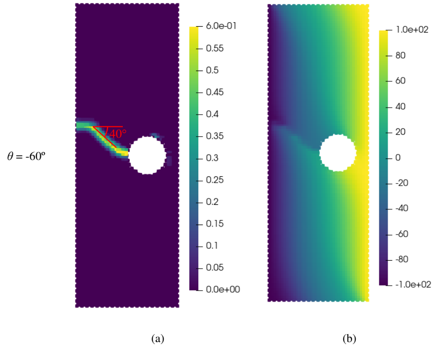
Fig. 6 Simulation results obtained by the proposed method for three cases with different material angles: (a) crack patterns; (b) temperature distributions (units: °C)
