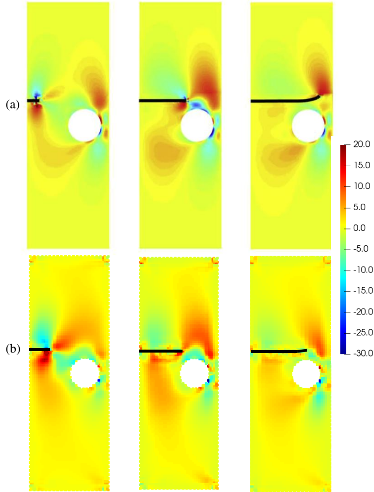
Fig.8 Distribution of shear stress obtained by different models with material angle \theta = 0^\circ : (a) extended four-node consecutive-interpolation element method (Nguyen et al., 2019); (b) the proposed method (units: MPa)
