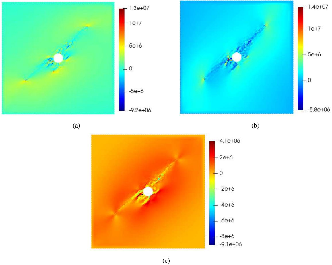
Fig.12 Contours of stress in an orthotropic rock specimen under high surrounding temperature with material angle \theta = 45^\circ : (a) horizontal stress; (b) vertical stress; (c) shear stress. (Units: Pa)
