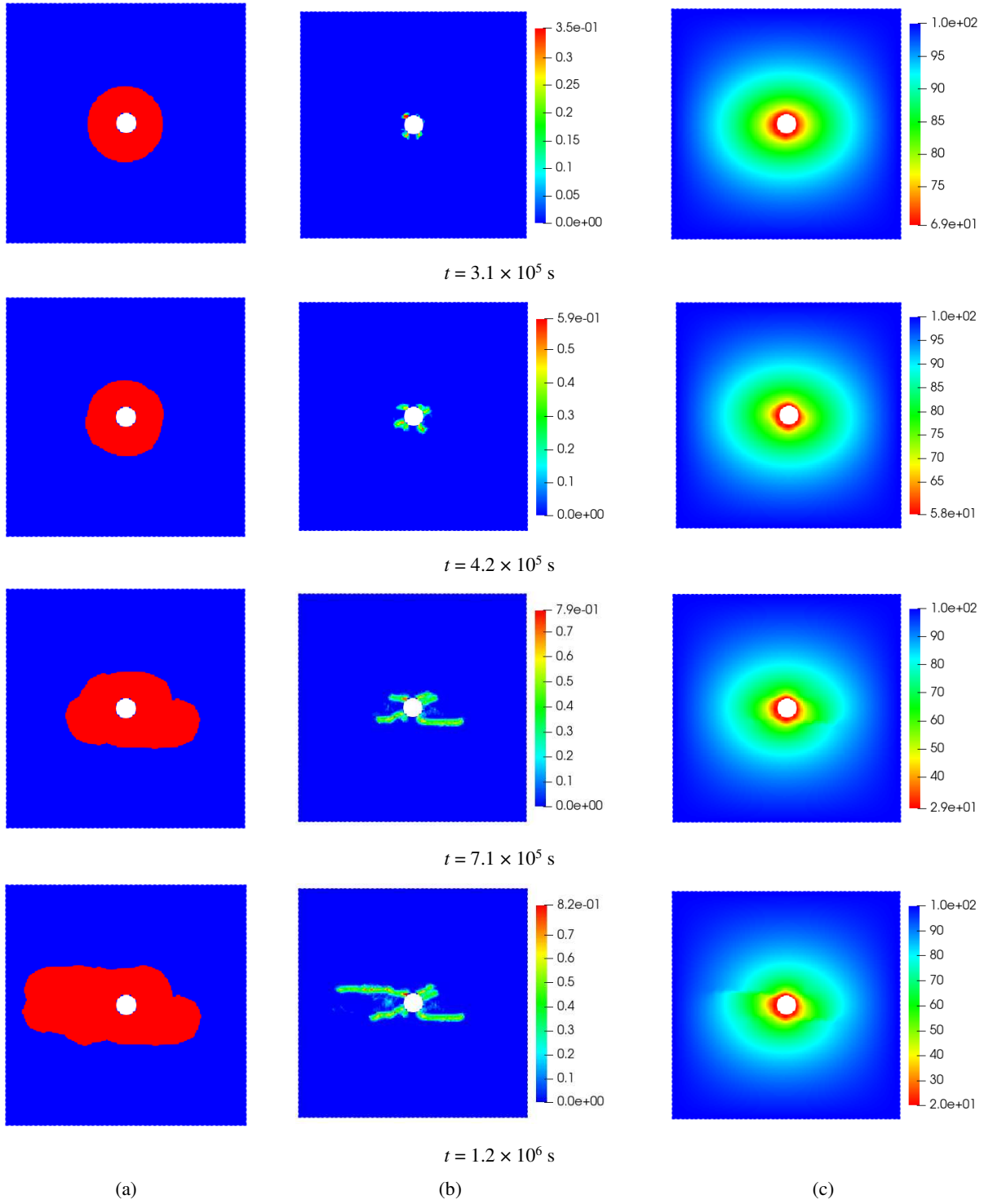
Fig 10 Thermal fracturing in an orthotropic rock specimen under high surrounding temperature using an adaptive scheme: (a) active PD particles drawing in red; (b) crack paths; (c) temperature distribution (units: °C)
