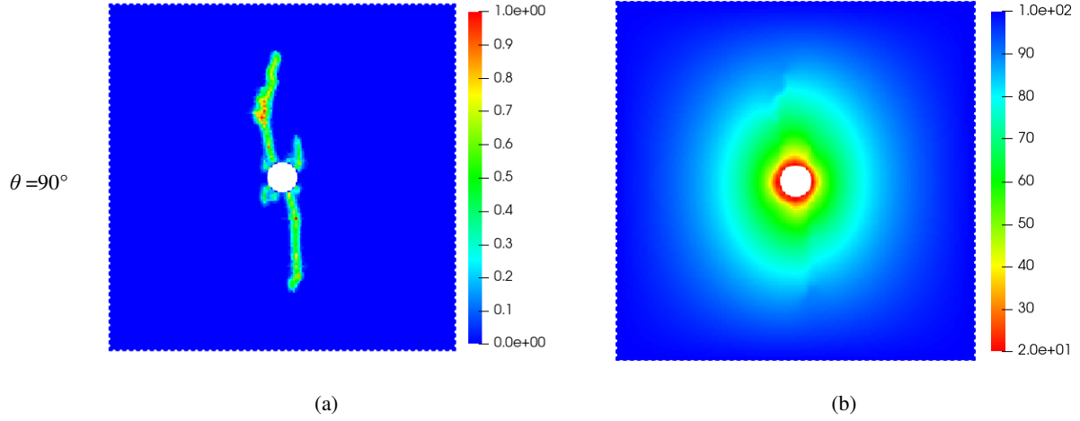
Fig.11 Thermal fracturing in an orthotropic rock specimen under high surrounding temperature with different material angles: (a) crack paths; (b) temperature distribution (units: ^\circ\text{C} )
