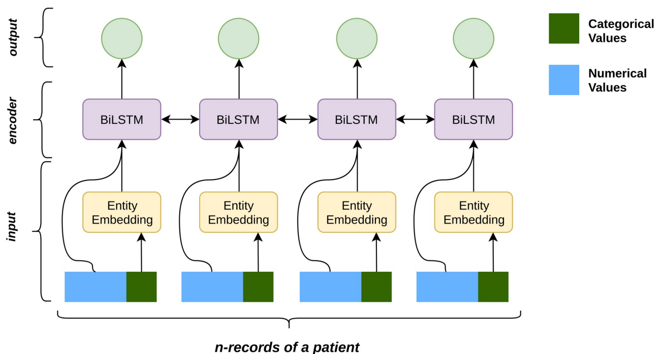
Fig 2. Model architecture.
