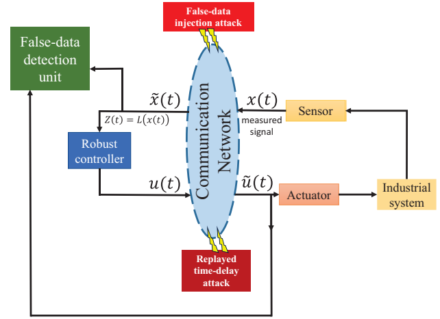
FIGURE 1 The structure of robust security control for a networked control system with false-data injection and replayed time-delay attacks
