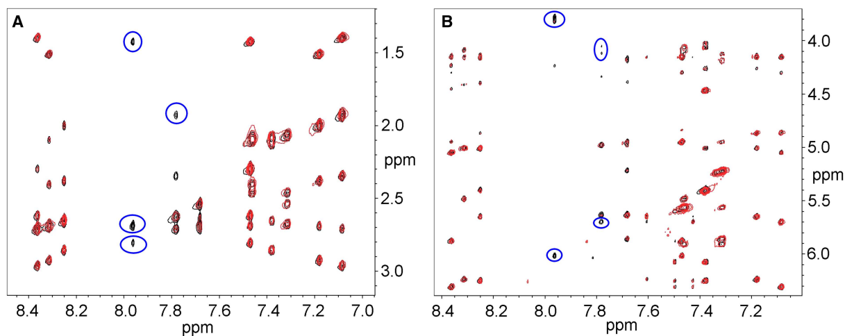
Figure 4. 2D NOESY spectra of 5 mM 12-mer B-DNA duplex.
