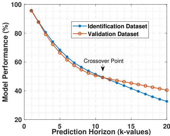
Fig. 6. The performance of the states space model with increasing prediction horizon. This indicates an exponential decay with a continuous rate of -0.085 per unit time of the model’s performance as k increases.
