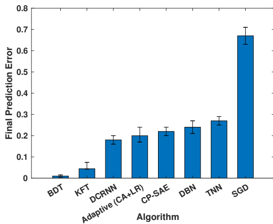
Fig. 10. Comparison of the eight different algorithms in terms of performance degradation (smaller values mean better performance).
