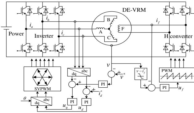
Fig. 3. Drive circuit for dual-excited VRM.
