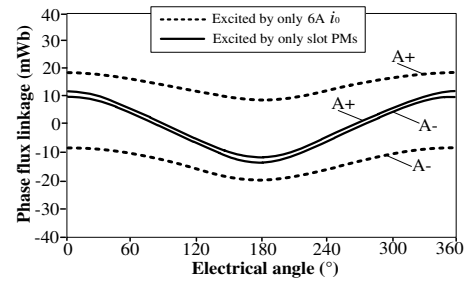
Fig. 10. No-load sub-phase flux linkage.
