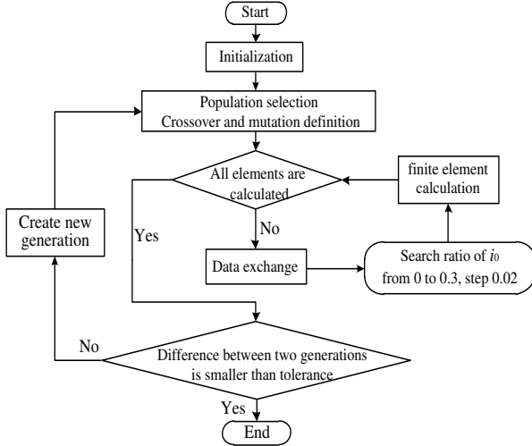
Fig. 25. Flowchart of the GA and Maxwell coupled optimization.
