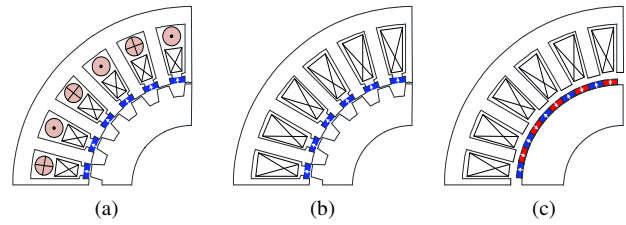
Fig. 27. (a) Existing VRM with separated AC and DC coils [22]. (b) Proposed VRM with integrated AC and DC coils. (c) Traditional SPM.
