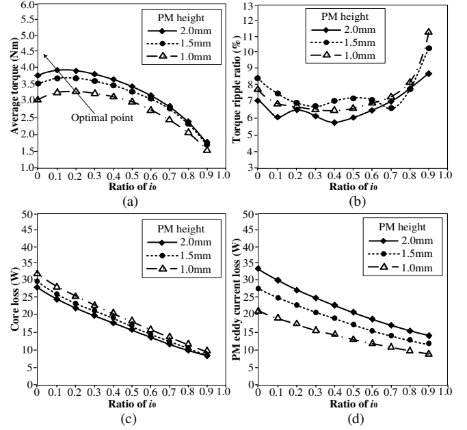
Fig. 23. Influence of PM height with different ratio of i_0 . (a) Average torque. (b) Torque ripple ratio. (c) Core loss. (d) PM eddy current loss.
