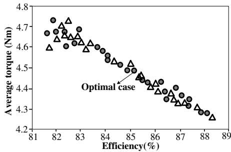
Fig. 26. Optimization results of last two generations.
