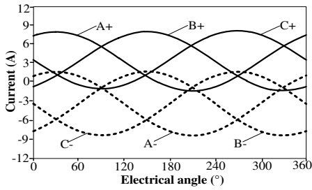
Fig. 14. Integrated AC and DC current excitation.
