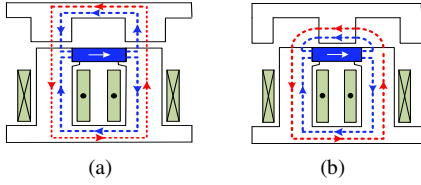
Fig. 6. No-load flux variation of Ap. (a) At d axis. (b) At q axis.
