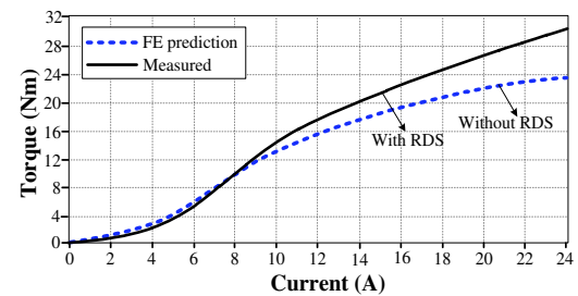
Fig. 30. Torque ability under different electrical load.
