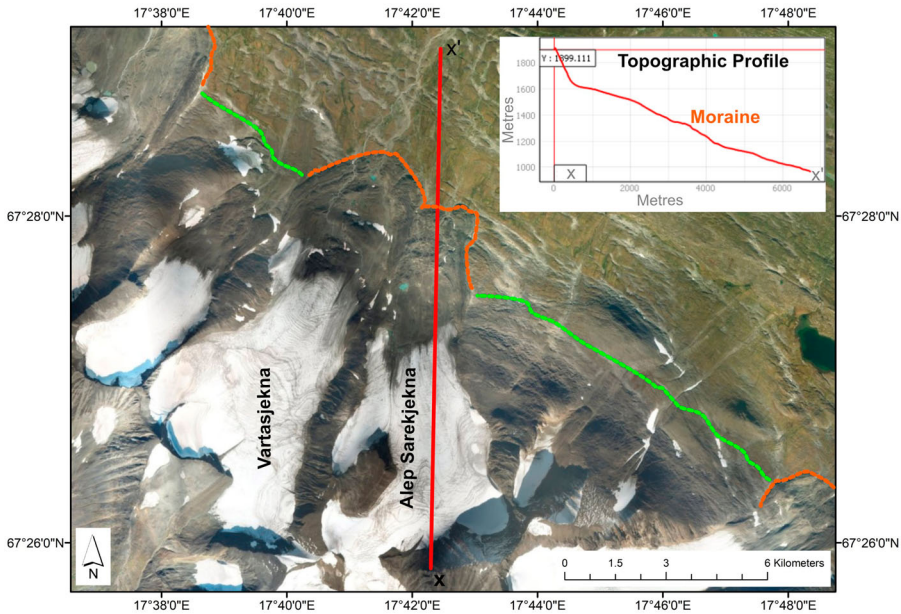
Figure 7. Satellite image from Digital Globe (WV2 0.5 m resolution) 30/8/2014 of Sarek area. The highest peak in the area, Sarektjokka (2,089 m) is in the bottom centre left of the image. Red line denotes the topographic profile (inset). Note the extensive terminal moraine systems (LIA maximum) extending beyond the corrie into the main valley below (orange dashed line). Green dashed line marks the valley side. Small proglacial lakes are clearly visible in the forefields due to the green colour from high suspended sediment load (Amphibolite). Orange dashed line = Little Ice Age Maximum.
