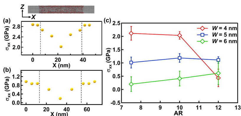
Figure 7. Sample stress distributions along Si NWs with an AR of 7.5 and W values of (a) 4 and (b) 6 nm. Significant tensile stresses are observed with their magnitude decreasing with increasing W . (c) MD prediction of average uniaxial stress in Si NWs as a function of AR. Stress level increases significantly with reducing W .
