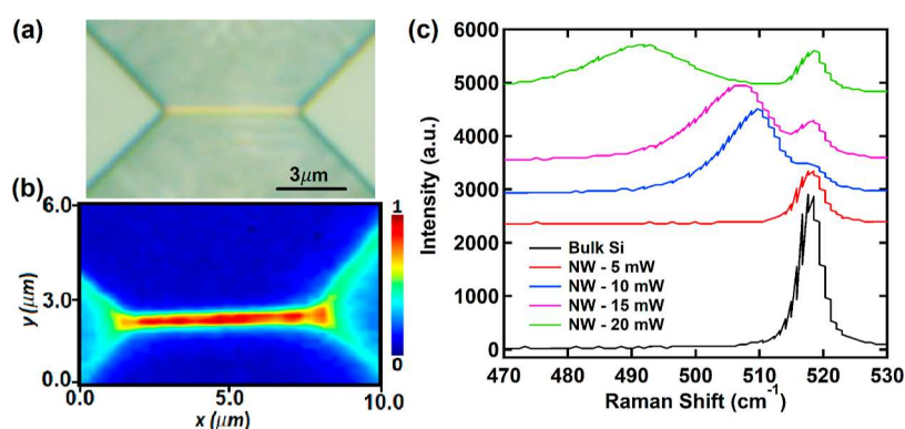
Figure 3. (a) Optical micrograph of a Si NW with a width of 80 nm and a length of 6 μm. (b) Mapped Raman intensity of the NW. (c) Raman spectra of bulk Si and the Si NW for a set of laser powers.
