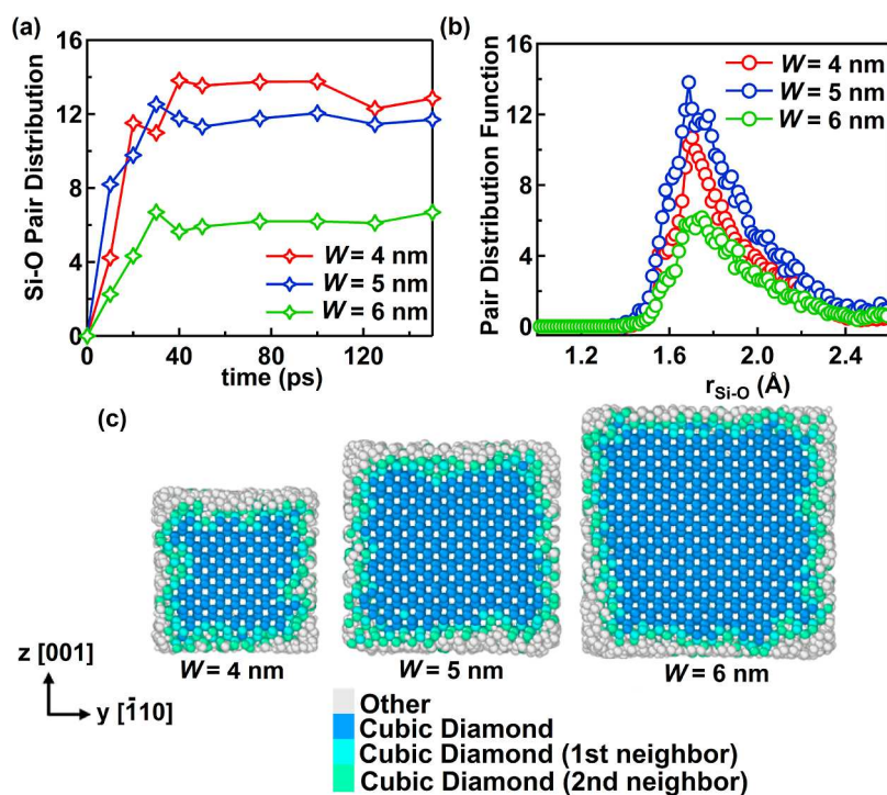
Figure 6. (a) Magnitude of the Si–O pair distribution as a function of time (AR = 7.5) and (b) PDF of Si–O for Si NWs at 40 ps. (c) Atomic structure of Si NWs upon oxidation. Diamond cubic crystal structure is retained within the crystalline core of the Si NW.
