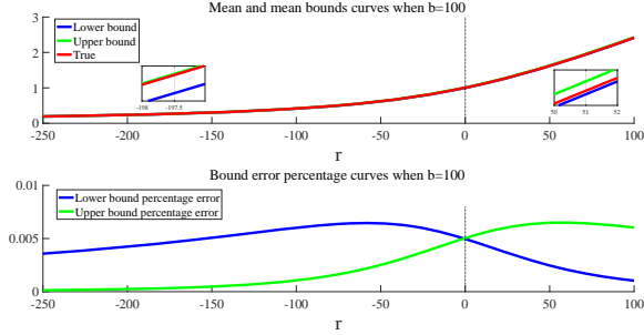
Fig. 4: Mean and mean bounds curves when b = 100 .
