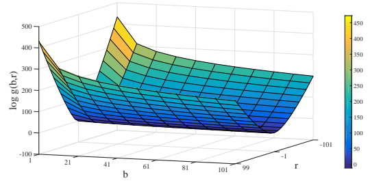
Fig. 3: The value of the logarithm of g(b, r) with respect to parameter b and r .
