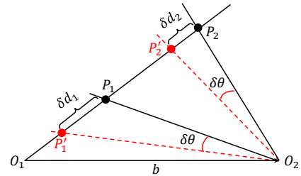
Fig. 1: Illustration for the time-varying MNCM caused by the triangulation. b denotes the baseline during two camera frames, and P_1 , P_2 denote the true position of the feature points, and P'_1 , P'_2 denote the positions estimated by the camera.
