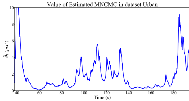
(b) Estimated MNCMC in the urban area.
