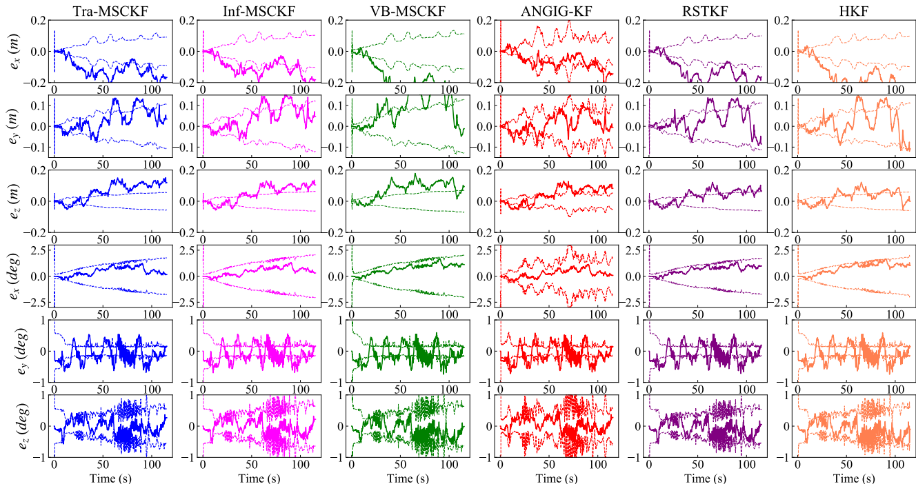
Fig. 14: 3-sigma bound curves of all algorithms for dataset V203.
