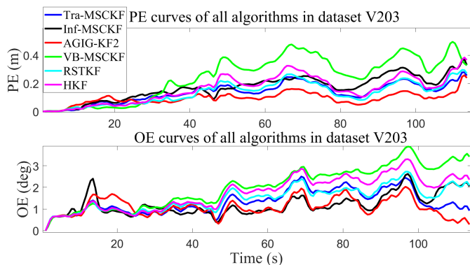
Fig. 12: PEs and OEs for dataset V203.
