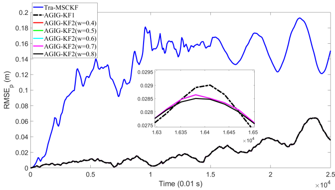
Fig. 11: PRMSEs of the proposed ANGIG-KF under different tuning weight \omega = 0.4, 0.5, 0.6, 0.7, 0.8 .
