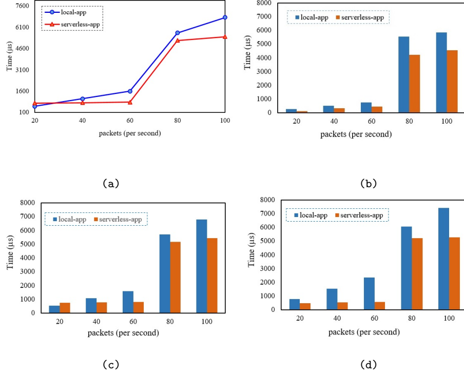
Fig. 3. The Average delay in: (a) different arrival rates. (b) service rate = \frac{1}{b} = 25\mu s . (c) service rate \frac{1}{b} = 34\mu s . (d) service rate \frac{1}{b} = 42\mu s .
