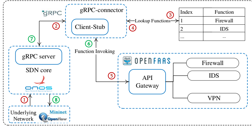
Fig. 2. ONOS and OpenFaaS Integration Sequence Diagram.
