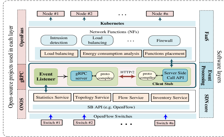
Fig. 1. A FaaS architecture for modular SDN.
