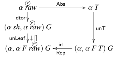
Fig. 3. The \text{raw} representation of T
