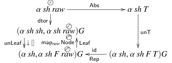
Fig. 4. Connecting the T - and the \text{raw} - components
