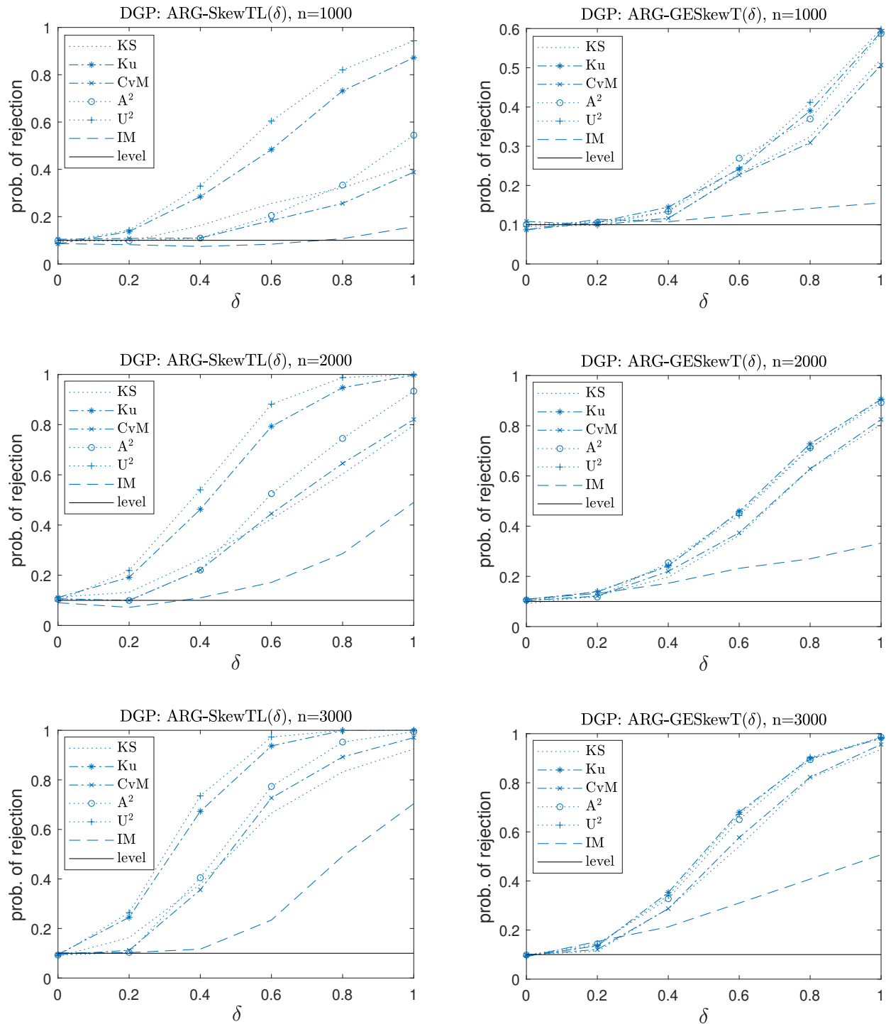
Figure 1: Empirical power curves at the 10% level. For panels on the left, the null hypothesis is ‘ H_0 : AR(1)-GARCH(1,1) with the error distribution being Skewed- t(v, \lambda) ’ and the DGP, denoted ARG-SkewTL( \delta ), is AR(1)-GARCH(1,1) with Skewed- t and Laplace mixture for which the pdf is f_{SkTL}(x) = (1 - \delta)f_{SkT}(x) + \delta f_L(x) . For panels on the right, the null hypothesis is ‘ H_0 : AR(1)-GARCH(1,1) model with the error distribution being GED(\theta) ’, and the DGP, denoted ARG-GESkewT( \delta ), is AR(1)-GARCH(1,1) with generalized-error and Skewed- t mixture distribution for which the pdf is f_{GESkT}(x) = (1 - \delta)f_{GE}(x) + \delta f_{SkT}(x) .
