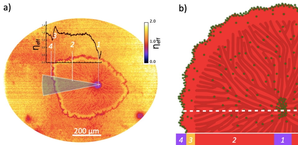
Fig. 4 (a) Map of photon multiplication performance for the TIPS-Tc:PbS-TET-CA ( 200 : 40 \text{ mg mL}^{-1} ) film, with insert showing radial sector integration across the crystalline feature. (b) Simplified schematic showing the different PbS-TET-CA QD morphologies/distributions within large TIPS-Tc crystallites. (1) A large QD aggregate at the nucleus of the feature. (2) A region of secondary crystallisation that has expelled remaining QD into relatively localised pockets. (3) A region where secondary crystallisation has not yet progressed, hence QD remain relatively well-dispersed (leading to a strip of enhanced photon multiplication performance). (4) The front comprising an aggregated ring of a large number of QD "swept" from the growing crystallite (leading to relatively poor photon multiplication performance). Surrounding the crystallite is the polycrystalline body of the film, beneath the size resolution of the present study.
