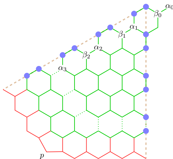
Figure 5: Fundamental region appropriate to an A_2 eigenvector of a(H(k+2, k, k, k)) with even k , shown explicitly for k = 6 . Blue filled circles indicate zero entries in the vector that are forced by symmetry. Green edges are present in both parent and altan; red edges are added in the altan. Mirror lines are shown in brown. Notation for variables \{\alpha_i\} and \{\beta_i\} is discussed in the text. Vertex p in the altan breaks the bipartite nature of this region, and allows determination of relationships between \{\alpha_i\} and \{\beta_i\} in the A_2 kernel eigenvector.
