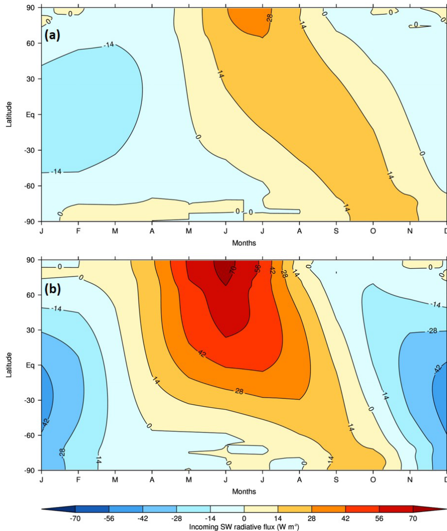
Figure 1. Calendar-adjusted latitude–month insolation (incoming SW radiative flux) anomalies: (a) midHolocene – piControl ; (b) lig127k – piControl .
