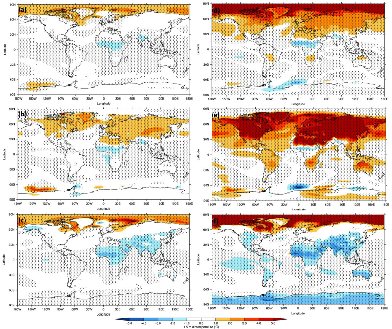
Figure 2. Calendar-adjusted 1.5 m air temperature climatology differences, HadGEM3 midHolocene and lig127k production runs versus HadGEM3 piControl production run: (a–c) midHolocene – piControl ; (d–f) lig127k – piControl . (a, d) Annual; (b, e) Northern Hemisphere summer (JJA); (c, f) Northern Hemisphere winter (DJF). Stippling shows statistical significance (as calculated by Student’s t test) at the 99 % level.
