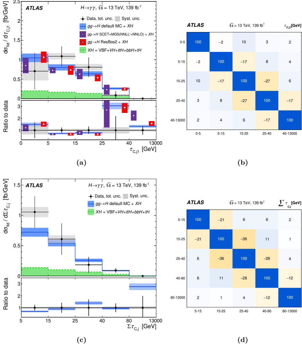
Figure 29. Particle-level fiducial differential cross-sections times branching ratio for the variables: (a) \tau_{C,j1} and (c) \sum \tau_{C,j} together with the corresponding correlation matrices ((b) and (d)).
