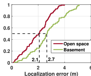
Fig. 20: CDF plots of the localization error.
