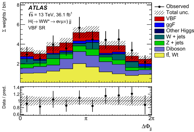
Fig. 7 The weighted \Delta\Phi_{jj} distribution in the VBF signal region, with signal and background yields fixed from the fit for \epsilon_{VV} using shape and rate information. Data-to-simulation ratios are shown at the bottom of the plot. The shaded areas depict the total uncertainty
