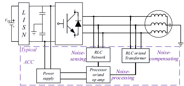
FIGURE 7. Schematic of the typical active EMI filter.
