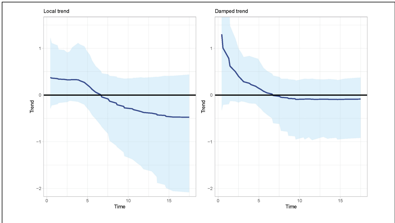
Figure 1 Estimates of the trend in the hazard function from 2 dynamic survival models. Solid blue line: point estimates, with 95% confidence intervals in pale blue. Black line: no trend.
