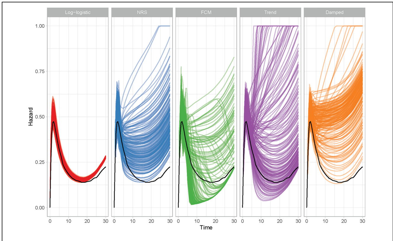
Figure 4 Relative survival model estimates of the hazard function and true values (black lines). FCM, flexible cure model; NRS, Nelson relative survival.
