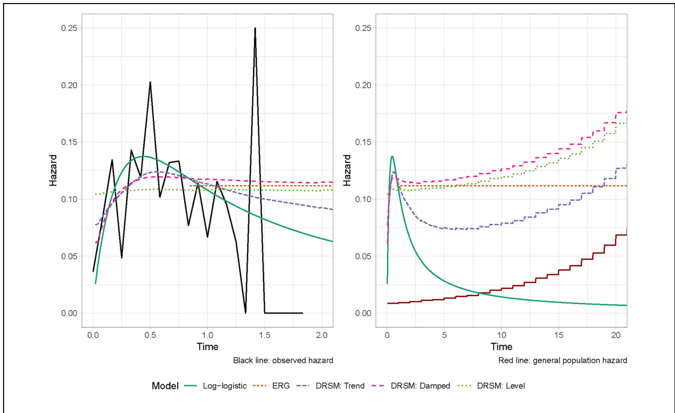
Figure 3 Hazard estimates with external data. Left: within-sample, right: extrapolations. Black line: observed hazard. Red line: general population hazard.
