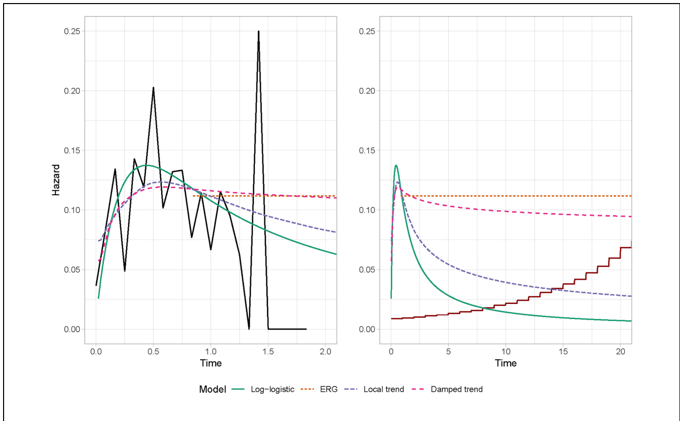
Figure 2 Hazard estimates without external data. Left: within-sample, right: extrapolations. Black line: observed hazard. Red line: general population hazard.
