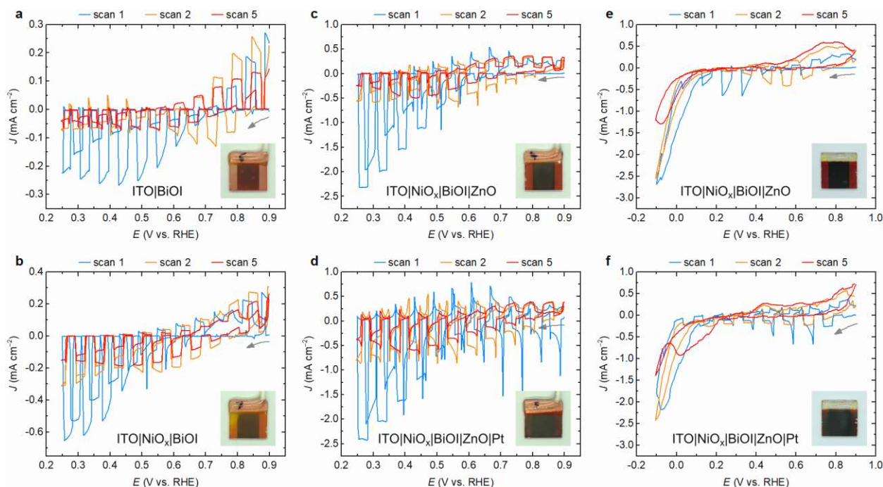
Supplementary Fig. 15 | Photoelectrochemical characterization of unprotected BiOI photocathodes. a, CVs of a bare ITO|BiOI photocathode. b, CVs of ITO|NiO x |BiOI. c,e, CVs of ITO|NiO x |BiOI|ZnO. d,f, CVs of ITO|NiO x |BiOI|ZnO|Pt. a-d – CVs are scanned between 0.9 and 0.25 V vs. RHE, with light chopped in 3 s on, 3 s off cycles. e,f – CVs are scanned between 0.9 and -0.1 V vs. RHE, with light chopped in 5 s on, 5 s off cycles. Grey arrows indicate the scan start and direction. Insets show the change in color of the photocathodes after 5 CV cycles (10 mV s -1 scan rate), which can be assigned to a partial BiOI reduction to a metallic Bi phase (see Supplementary Fig. 14). This change is only observed for BiOI deposited above the patterned ITO stripe. Similar degradation patterns are observed both in the presence and absence of the 5 nm Pt layer, indicating that the Bi reduction is not caused by insufficient charge extraction / charge accumulation. An increased dark current can be observed in frames e and f , as BiOI electroreduction occurs at applied potentials below 0.2 V vs. RHE. The photocurrent was significantly diminished over subsequent scans for all samples, as BiOI reduction occurred during the first CV cycle (see Supplementary Movie 2). No H 2 was detected over the five cycles for samples in a-d , which indicates the photocurrent is solely caused by BiOI reduction. An anodic photocurrent was only observed after the BiOI reduction over the first scan (Supplementary Fig. 16), which indicates the current is due to Bi reoxidation. CVs were conducted under chopped light irradiation (AM 1.5G, 100 mW cm -2 ), in 0.1 M KBi, 0.1 M K 2 SO 4 , pH 8.50, under N 2 , at room temperature.
