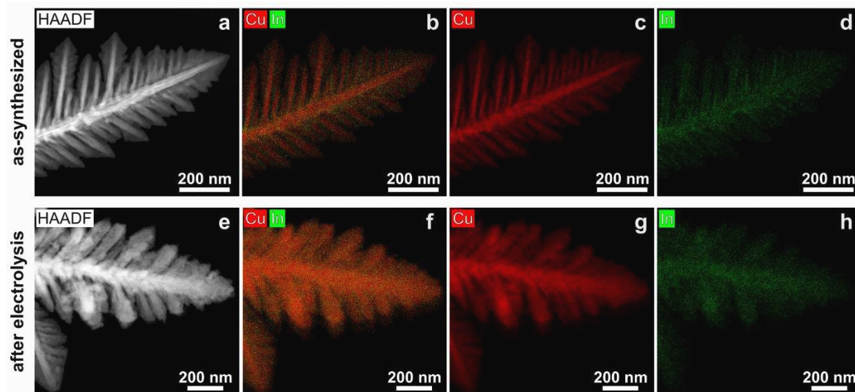
Supplementary Fig. 24 | Pre- and post-catalysis HAADF and STEM mapping of the \text{Cu}_{92}\text{In}_8 alloy electrocatalyst. a,e , High-angle annular dark-field (HAADF) images. b-d,f-h , Scanning transmission electron microscopy (STEM) elemental mapping depicting overall ( b,f ), copper ( c,g ) and indium ( d,h ) distributions. Data is obtained prior ( a-d ) and after ( e-h ) the long-term \text{CO}_2 reduction experiment described in Supplementary Fig. 23. The dendritic \text{CuIn} alloy undergoes an in situ phase transformation during operation where the In phase gradually migrates into the bulk of the dendrites. This process exposes the Cu phase on the catalyst surface, which is mainly active towards \text{H}_2 evolution under the experimental conditions 5 .
