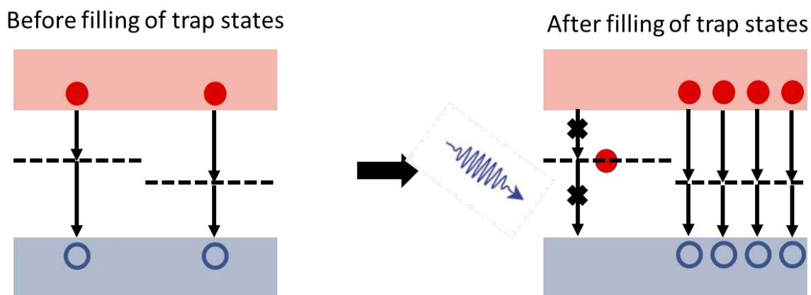
Supplementary Fig. 38 | Schematic showing the effect of light soaking on the recombination kinetics. Before prolonged light exposure all defect states are unoccupied (left part). After prolonged light exposure trap states are filled (right part) reducing the recombination rate, increasing the carrier density, and open circuit voltage.
