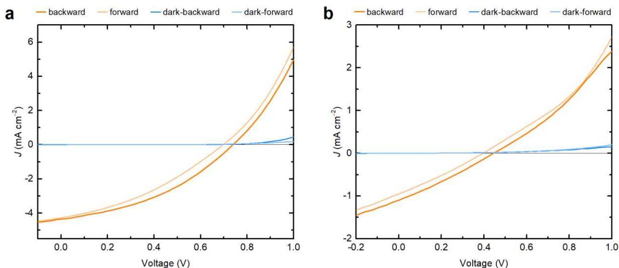
Supplementary Fig. 5 | Examples of forward and backward J - V curves for BiOI PV devices of different sizes. a , One representative 0.045 cm 2 pixel from an 8-pixel device. b , One-pixel 0.25 cm 2 device. Despite the difference in V_{OC} and J_{SC} , the relative hysteresis between forward and backward scans remains similar for both sizes.
