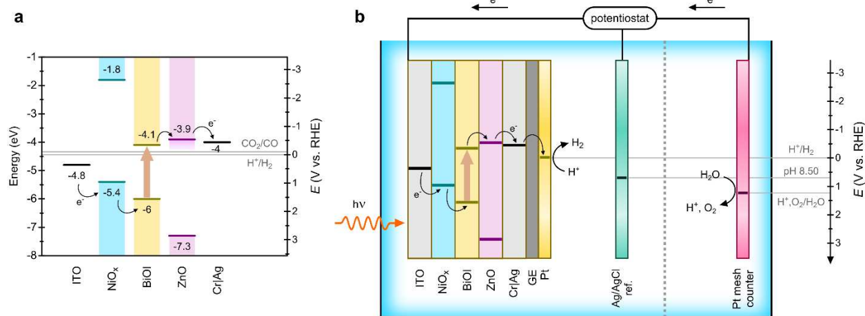
Supplementary Fig. 8 | Band structures of the BiOI PV cells and photocathodes. a , Energy levels within a BiOI PV device. b , Schematic of the energy levels of a BiOI photocathode in solution, wired in a three-electrode configuration with a Ag/AgCl/NaCl(sat.) reference electrode, and a Pt mesh counter electrode. Owing to its intrinsic nature, BiOI has a low carrier concentration and therefore will have a large depletion width when deposited onto n - or p -type substrates. When BiOI is sandwiched between NiO x and ZnO a built-in potential is created, which under short-circuit conditions cause electrons to get injected into the ZnO and directed towards the Cr|Ag contact. Whilst the electron affinity of ZnO is lower than that of BiOI, electrons can still be injected into the tail of states extending from the conduction band minimum of ZnO and into the bandgap, meaning that there is no extraction barrier (see absorption and photoluminescence spectra of ZnO in Supplementary Fig. 9). These electrons are transferred through the conductive graphite epoxy (i.e. ohmic contact) to either a Pt or Cu 2 In 8 catalyst. The BiOI photocathode is therefore capable of both hydrogen evolution and CO 2 reduction.
