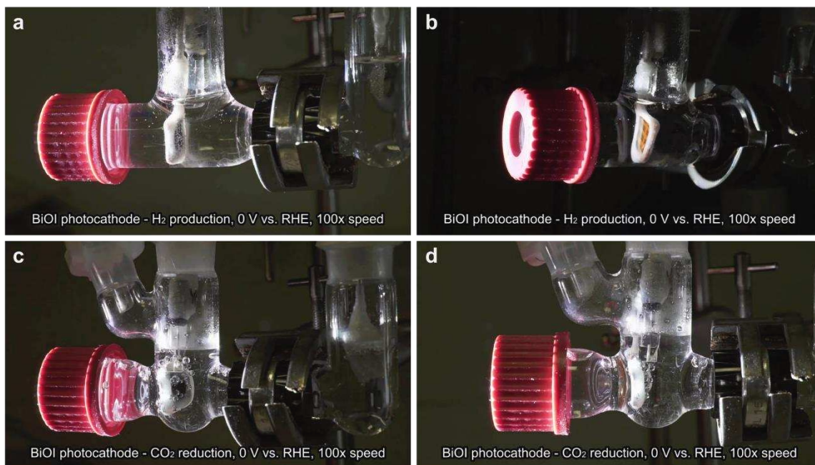
Supplementary Fig. 41 | Snapshots from Supplementary Movie 1 of BiOI photocathodes under operation in a three-electrode system. a,b , Photocathodes with a Pt catalyst for H 2 evolution. c,d , Photocathodes with a Cu 92 In 8 catalyst for CO 2 reduction to syngas. The stability tests are performed at an applied potential of 0 V vs. RHE. The movie speed is increased to highlight the bubble formation.
