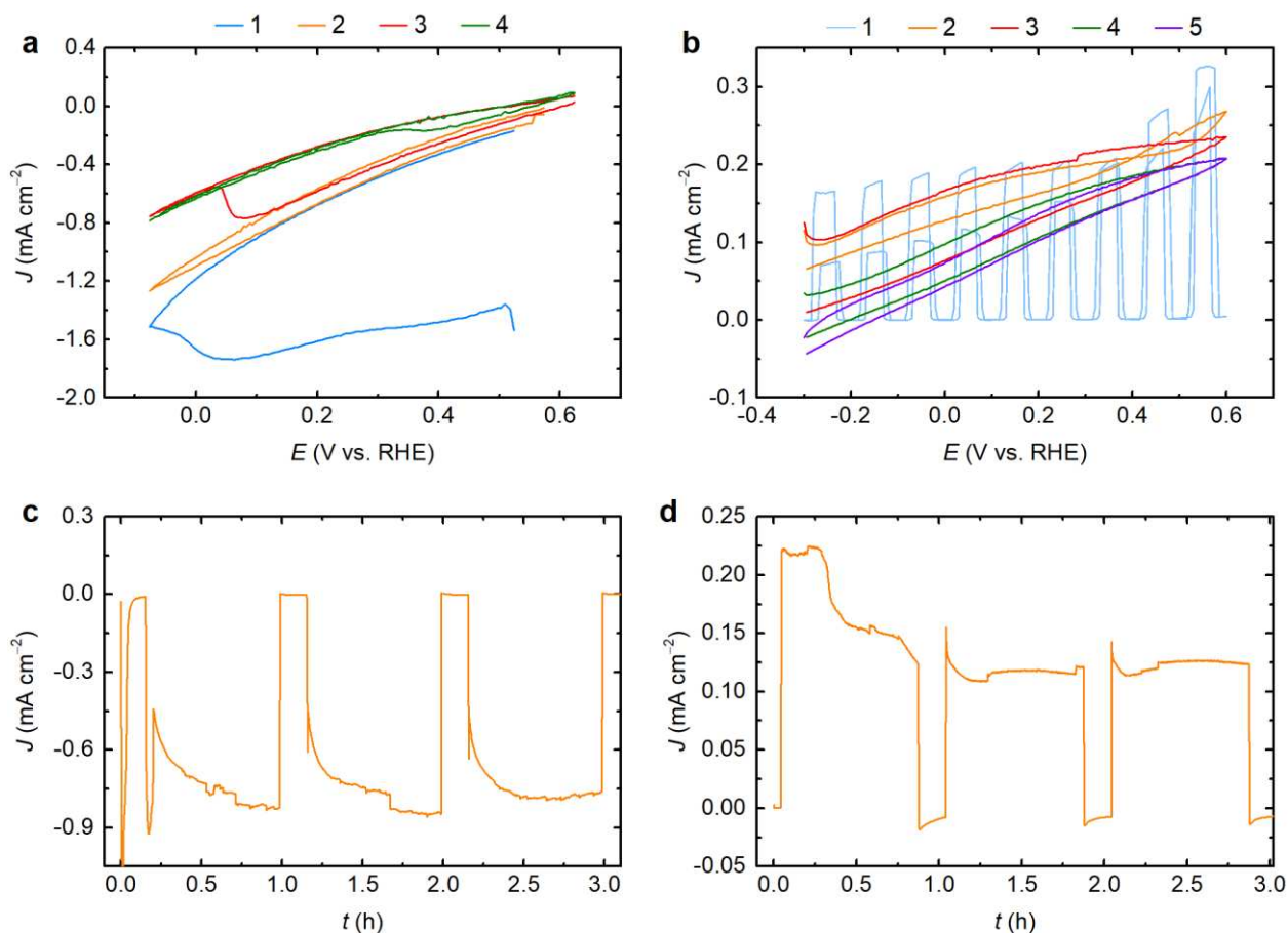
Supplementary Fig. 28 | Reduction of the Cu 2 O phase from the Cu 92 In 8 catalyst surface during PEC operation. a,c, BiOI|GE|Cu 92 In 8 photocathodes. b,d, BiOI|GE|Cu 92 In 8 - BiVO 4 tandem devices. Due to an aerial oxidation, a minor Cu(I) oxide phase (Cu 2 O) appears on the nanodendritic catalyst surface (see Supplementary Fig. 27). Under photoelectrochemical conditions, this oxide layer is rapidly reduced back to metallic Cu. Thus, during operation, the active catalyst is pure metallic Cu 92 In 8 alloy which does not contain any oxide component. This oxide reduction can be observed through an increased photocurrent in the cyclic voltammograms of the photocathodes and tandem devices which disappears after 3-5 cycles (a,b), or through a high initial photocurrent within the first 30 min in chronoamperometry, before reaching steady state (c,d).
