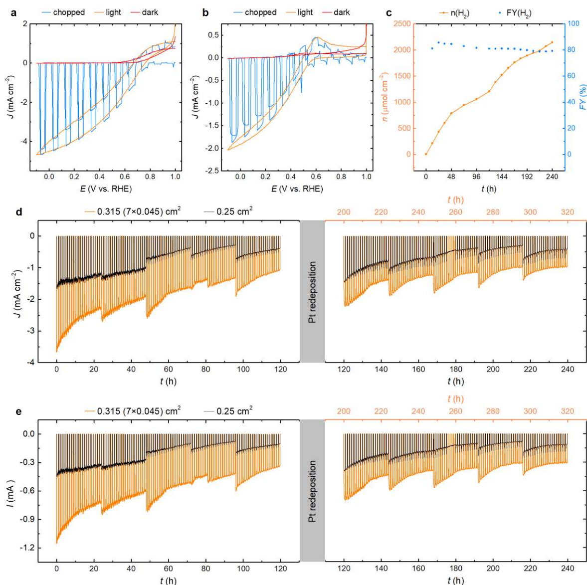
Supplementary Fig. 11 | Photoelectrochemical characterization of the BiOI|GE|Pt photocathodes. a , Cyclic voltammetry (CV) scans of a photocathode consisting of seven 0.045 \text{ cm}^2 working BiOI pixels (i.e. 0.315 \text{ cm}^2 photoactive area) under chopped, continuous and no light irradiation. b , CV scans of a 0.25 \text{ cm}^2 one-pixel photocathode. c , Close-up of the \text{H}_2 evolution over time for the 0.25 \text{ cm}^2 electrode. d , Comparison of the photocurrent decay over time and recovery after Pt redeposition for the 0.315 (7 \times 0.045) \text{ cm}^2 and 0.25 \text{ cm}^2 photocathodes. While the absolute decay rates are comparable, the relative decrease in photocurrent is higher for the 0.25 \text{ cm}^2 photocathode due to its smaller photocurrent density. A partial recovery in respect to the initial photocurrent is observed in both cases ( 7 \times 0.045 and 0.25 \text{ cm}^2 ) when redepositing 5 \text{ nm} Pt, irrespective of the prior operation time (200 vs. 120 h), or resting time in between long-term tests (21 vs. 0 days, respectively). Experiments are conducted under simulated solar irradiation ( \text{AM } 1.5\text{G} , 100 \text{ mW cm}^{-2} ), in 0.1 \text{ M KBi} , 0.1 \text{ M K}_2\text{SO}_4 , \text{pH } 8.50 , under \text{N}_2 , at room temperature. e , Absolute photocurrents for the two photocathodes described in frame d . The 0.315 (7 \times 0.045) \text{ cm}^2 photocathode presents a roughly 2.5 times higher absolute photocurrent than a 0.25 \text{ cm}^2 single pixel electrode, even though both devices are fabricated on substrates of the same total area ( 1.2 \times 1.2 \text{ cm}^2 ). Hence, the photocurrent of multiple-pixel devices also surpasses single-pixel electrodes when considered over the entire device area.
