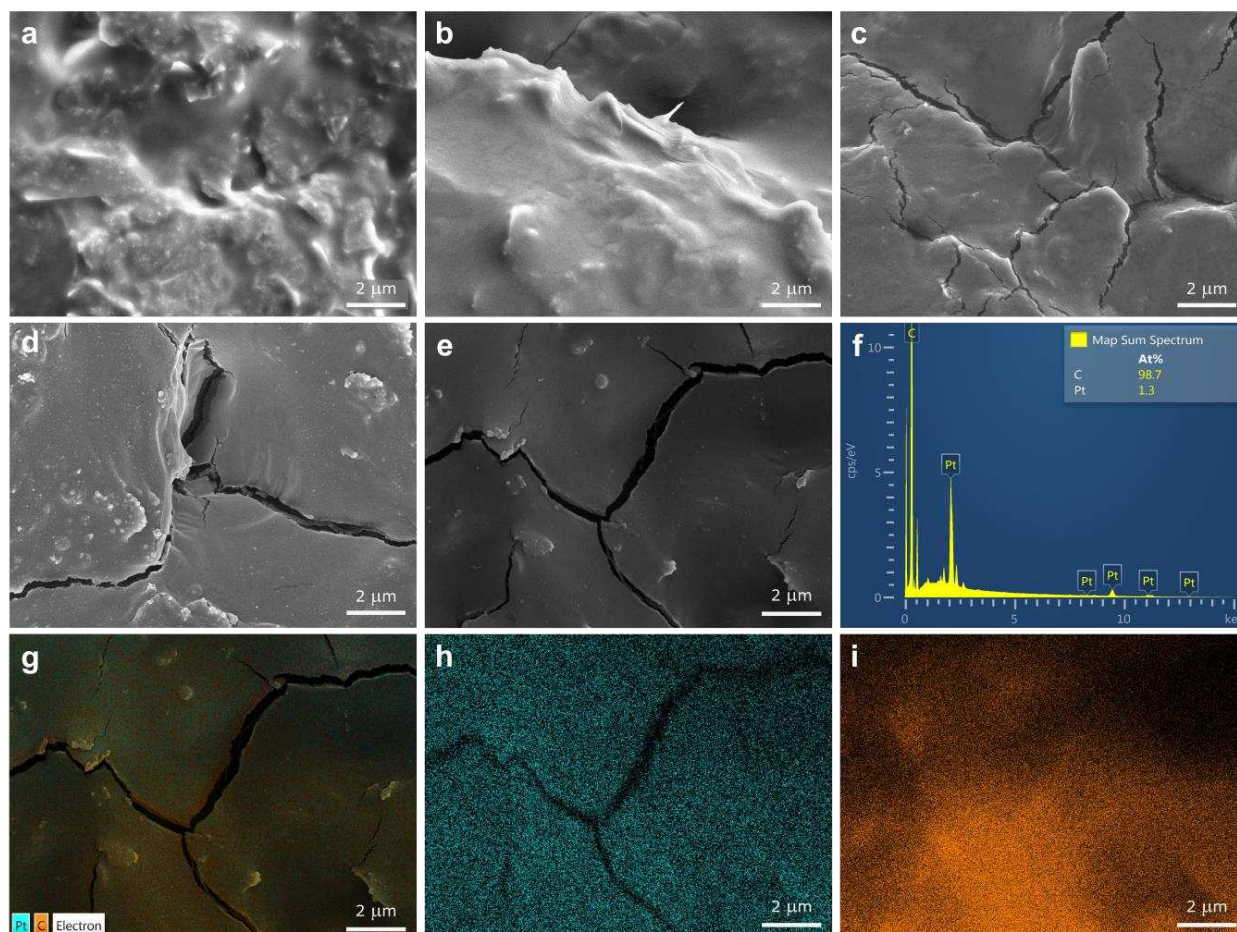
Supplementary Fig. 17 | Degradation of the GE|Pt electrocatalyst surface over the 500 h BiOI|GE|Pt photocathode test. a-e, SEM images. a, Pristine GE surface. b, Fresh GE|Pt electrocatalyst. c, GE|Pt catalyst after a 120 h electrolysis test (Supplementary Fig. 18a). d,e, GE|Pt surface after the 500 h photocathode test (Fig. 2b, main text). f, EDX spectrum corresponding to the area depicted in frame e. g-i, Overall (g), platinum (h) and carbon (i) elemental mapping. As observed previously, a decrease in activity of the Pt catalyst is caused by nano-cracks forming over the GE|Pt catalyst interface which may affect the electronic transport, whereas only a minimal amount of Pt (below 1%) becomes detached from the electrode surface 4 .
