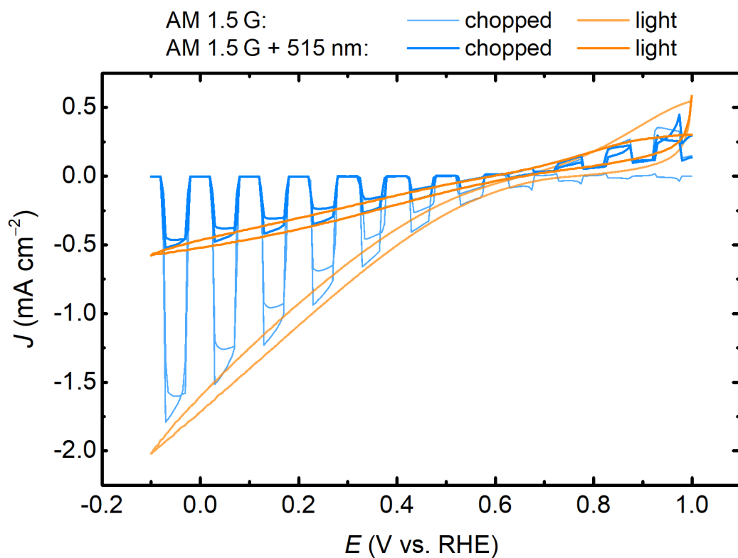
Supplementary Fig. 36 | CVs of a BiOI|GE|Pt photocathode. Measured under 1 sun irradiation (AM 1.5G, 100 \text{ mW cm}^{-2} , in 0.1 \text{ M KBi} , 0.1 \text{ M K}_2\text{SO}_4 , pH 8.50, under \text{N}_2 ), with or without a 515 nm cut-off filter. The 515 nm light filtering results in significantly lower photocurrent densities, which resemble the photocurrents displayed by tandem devices (i.e. with BiOI behind \text{BiVO}_4 ).
