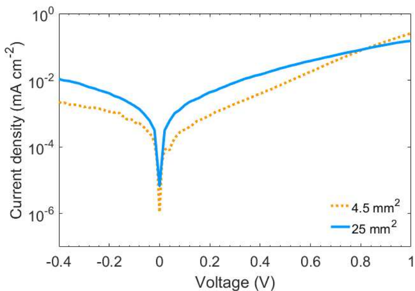
Supplementary Fig. 4 | Dark current density of two BiOI PV devices. The active areas are 4.5 mm 2 (yellow dashed line) and 25 mm 2 (blue solid line).
