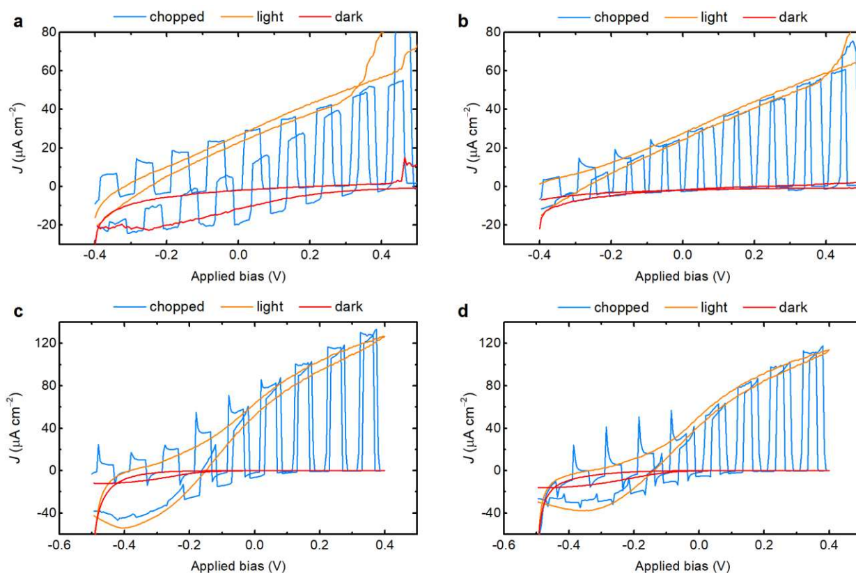
Supplementary Fig. 37 | Trap filling behavior of the BiOI|GE|Pt - BiVO 4 tandem devices during operation. a,b , CVs of a 0.225 (5×0.045) cm 2 BiOI - 0.25 cm 2 BiVO 4 tandem recorded before (a) and after (b) 12 h chronoamperometry (CA) at 0 V applied bias. c,d , CVs of a 0.25 cm 2 BiOI - 0.25 cm 2 BiVO 4 tandem recorded before (c) and after (d) 12 h CA. Instead of promoting device degradation, the prolonged light exposure leads to a decrease in the dark current (b, d) and an increase of the device photovoltage (see earlier onset voltage for water splitting in b). This may be explained by a trap filling mechanism, which manifests through an increase in V oc during light soaking of the devices (see Supplementary Fig. 39). Experiments are performed under simulated 1 sun irradiation (AM 1.5G, 100 mW cm -2 ), in 0.1 M KBi, 0.1 M K 2 SO 4 , pH 8.50, under N 2 .
