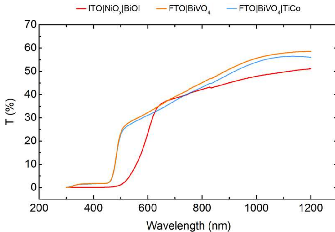
Supplementary Fig. 34 | UV-vis transmittance spectra of BiOI and BiVO 4 . The front BiVO 4 photoanode can absorb light up to 500 nm, leaving a small part of the solar spectrum available for the BiOI light absorber. The thin, transparent TiCo water oxidation catalyst does not have a significant effect on the transparency of the BiVO 4 photoanode.
