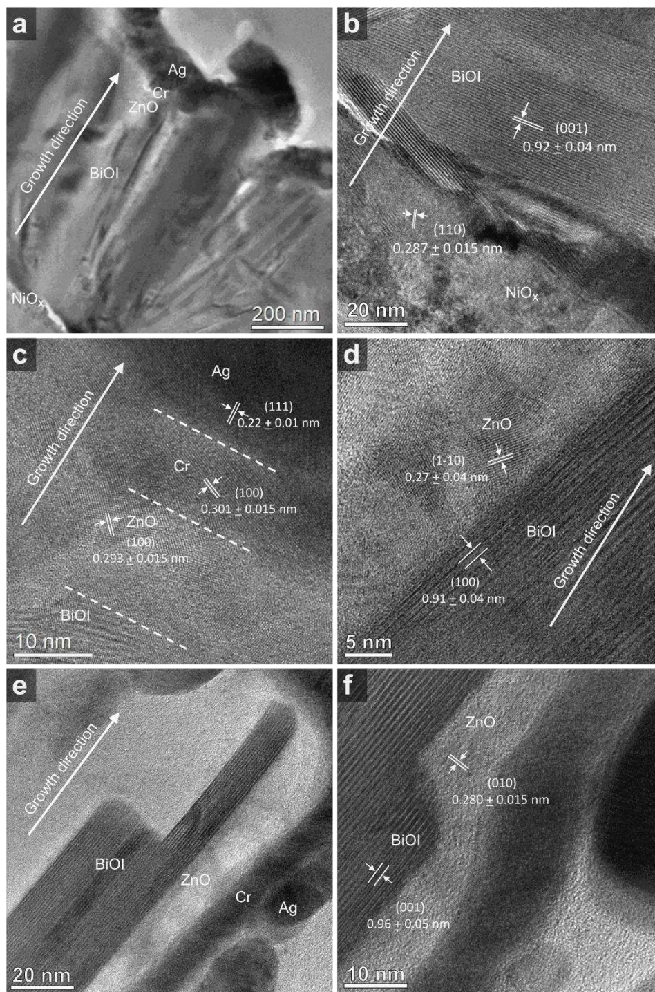
Supplementary Fig. 1 | TEM images of NiO x |BiOI|ZnO|Cr|Ag solar cells on Si substrates. a , Bright field TEM overview image obtained by FIB milling shows the full BiOI PV device structure along the growth direction, including the substrate, NiO x , BiOI, ZnO, Cr and Ag contact (n.b. the growth direction denotes the normal to the substrate). b , High resolution TEM (HRTEM) image of the interface between the NiO x hole transport layer and the BiOI light absorber, revealing the polycrystalline nature of both NiO x nanograins and BiOI platelets. The (100) and (110) atomic planes of BiOI and NiO x are outlined, respectively. c , HRTEM image of the ZnO, Cr and Ag layers. Lattice spacing analysis was used to identify different layers and label characteristic atomic planes. d , HRTEM image of the interface between the ZnO electron selective layer and a platelet of BiOI. e,f , HRTEM image of a BiOI platelet with the ZnO, Cr and Ag layers. Here it is visible that the ZnO deposited by atmospheric pressure chemical vapor deposition conformally coats the BiOI platelets.
