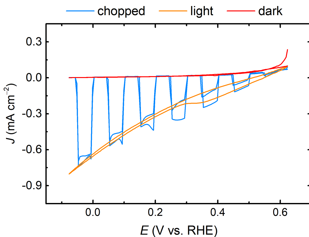
Supplementary Fig. 29 | Cyclic voltammetry scans of a 0.27 (6×0.045) cm 2 BiOI|GE|Cu 92 In 8 photocathode for CO 2 reduction, under chopped, continuous and no light irradiation. Light experiments are performed under 1 sun irradiation (AM1.5G, 100 mW cm -2 ), in a 0.5 M KHCO 3 electrolyte solution, under CO 2 , pH 7.4.
