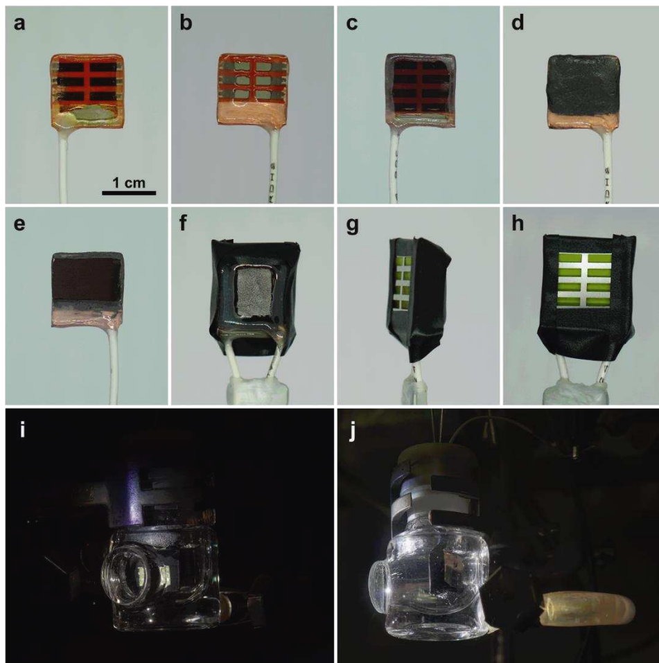
Supplementary Fig. 40 | Photographs of the BiOI devices during encapsulation and operation. a-e , Intermediate steps in the BiOI photocathode encapsulation: a,b - wiring and insulating the active areas using epoxy resin; c,d - applying the graphite epoxy paste as conductive encapsulant; e - attachment of a Cu foil with a dendritic \text{Cu}_{92}\text{In}_8 foam catalyst onto the fresh graphite paste. f,g,h , Close-up images of the masked 0.315 (7 \times 0.045) \text{ cm}^2 BiOI - 0.52 (8 \times 0.065) \text{ cm}^2 \text{BiVO}_4 tandem device. i,j , Photographs of the wired tandem device under operation in a one-compartment PEC cell.
