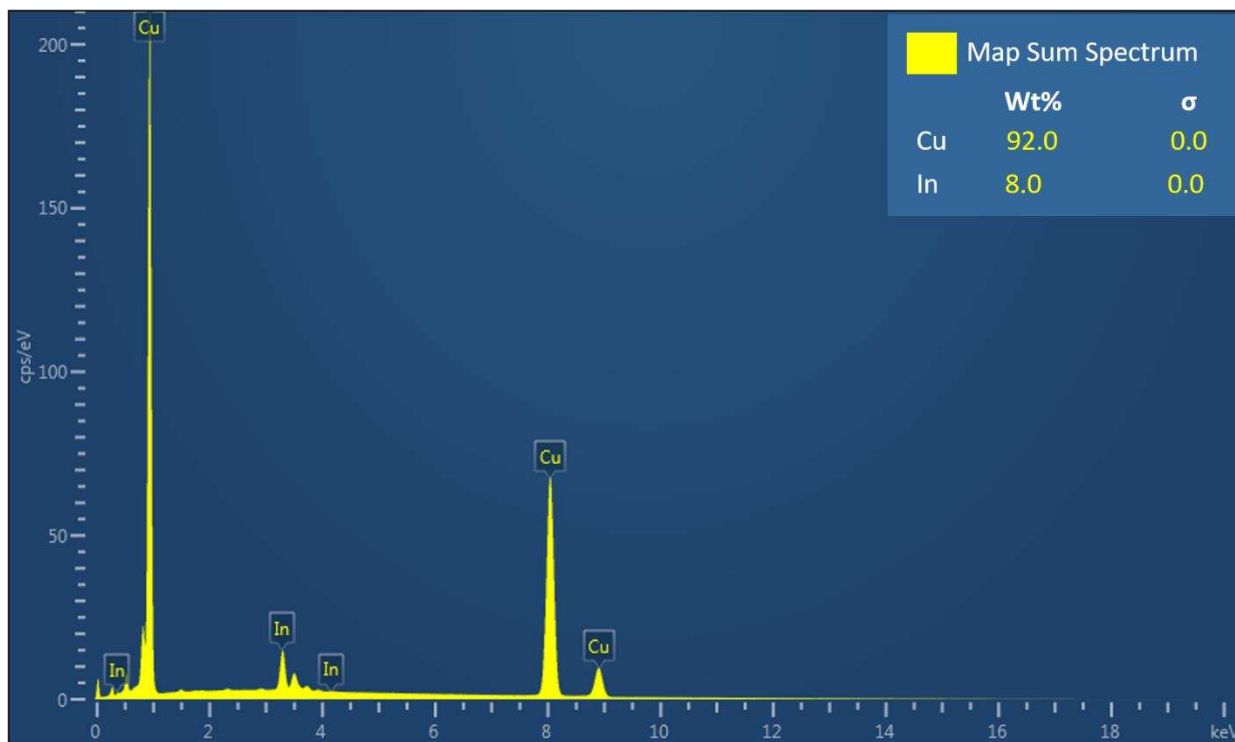
Supplementary Fig. 26 | EDX analysis confirms the composition of the \text{Cu}_{92}\text{In}_8 alloy employed for \text{CO}_2 reduction.
