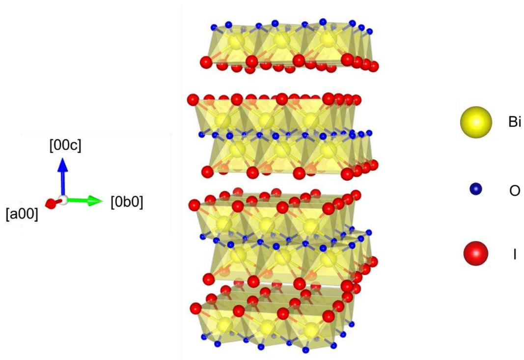
Supplementary Fig. 2 | Crystal structure of bismuth oxyiodide. The crystallographic axes are depicted on the left, the labels for the atoms on the right. There are 3 \times 3 \times 3 unit cells depicted.
