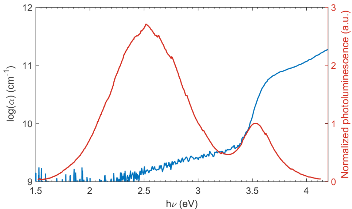
Supplementary Fig. 9 | Absorption and photoluminescence (PL) spectra of ZnO. The ZnO films grown here were deposited at a low temperature of 80 °C, and therefore have many defects and high levels of disorder. This results in a high density of tail states extending from the band-edges. Charges can be injected into these tail states. In our case, electrons from BiOI can be injected 0.3 eV below the conduction band minimum, where the density of electron acceptor states is sufficient to sustain photocurrents without presenting a charge extraction barrier 1 . Figure adapted with permission from Ref. 2.
