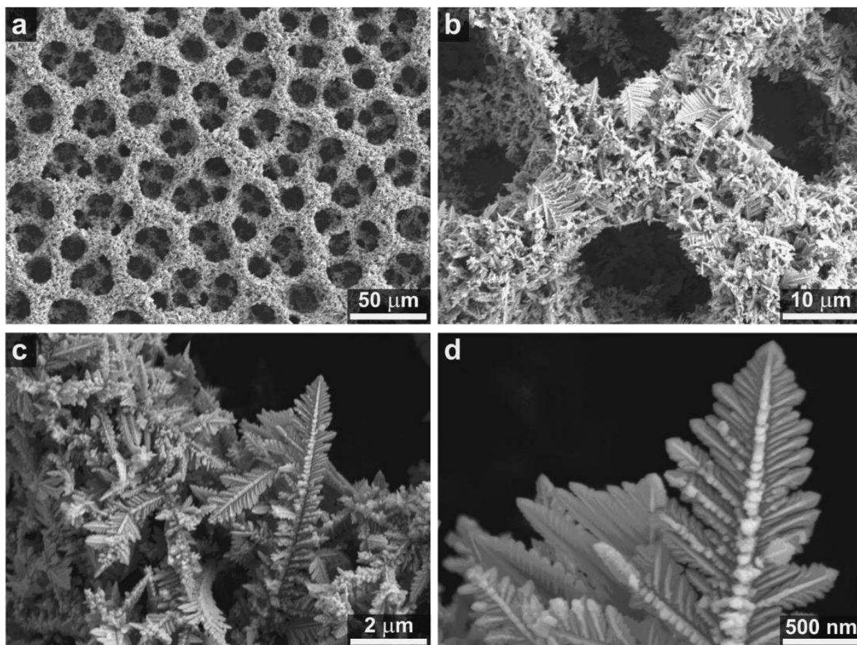
Supplementary Fig. 25 | SEM and HR-SEM analysis of the \text{Cu}_{92}\text{In}_8 alloy electrocatalyst at different magnifications. a-d, The catalyst displays a dendritic foam morphology, which enables it to attain a high selectivity towards \text{CO}_2 reduction at a low overpotential.
