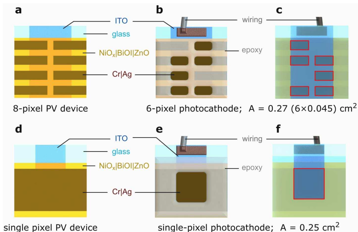
Supplementary Fig. 12 | Photoactive areas for different PV and PEC pixel arrangements. a,b,c , Multiple-pixel arrangement. d,e,f , Single-pixel design. a,d , PV devices. b,c,e,f , Partially encapsulated photocathodes, seen from: b,e - the front side, c,f - the back side (corresponding to the images in Supplementary Fig. 40a,b). In case of the multiple-pixel arrangement, eight independently working, 0.045 \text{ cm}^2 PV cells are defined by evaporating metal Cr/Ag contacts onto a 1.2 \times 1.2 \text{ cm}^2 substrate through a mask. Each substrate forms the basis for a multiple-pixel photocathode. In example b , six working pixels are selected for the photocathode, whereas two faulty pixels and the remaining non-active area are sealed by epoxy. The six working pixels are connected in parallel via the conductive graphite epoxy paste (see Supplementary Fig. 40b,d), resulting in an electrode with a total photoactive area of 6 \times 0.045 \text{ cm}^2 = 0.27 \text{ cm}^2 (see red highlights). In this multiple-pixel arrangement, the photocathode maintains the higher voltage of the small-area pixels, while the absolute photocurrents add up (i.e. the overall photocurrent density remains similar). In contrast, only one 0.25 \text{ cm}^2 PV cell is deposited on the 1.2 \times 1.2 \text{ cm}^2 substrate in case of the single-pixel devices, with its photoactive area defined by the size of the conductive ITO stripe (see f ). The non-active area is again sealed by epoxy when assembling the photocathode.
