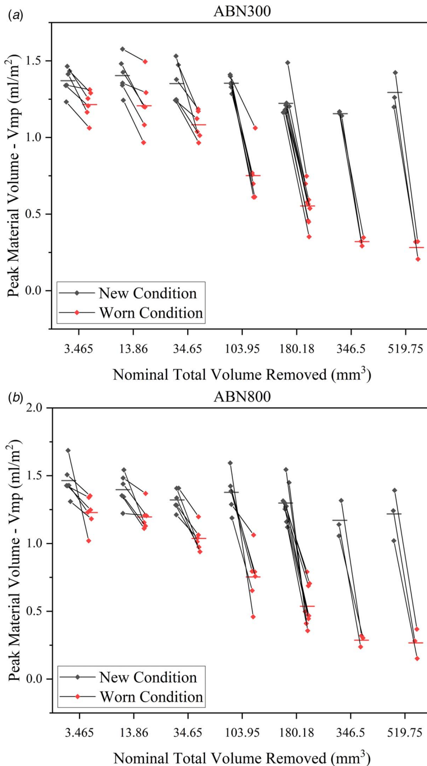
Fig. 17 Comparison of matching new and worn condition surface peak material volumes ( V_{mp} ) from three sides of the same tool following point grinding using (a) ABN300 and (b) ABN800 abrasive under various durations
