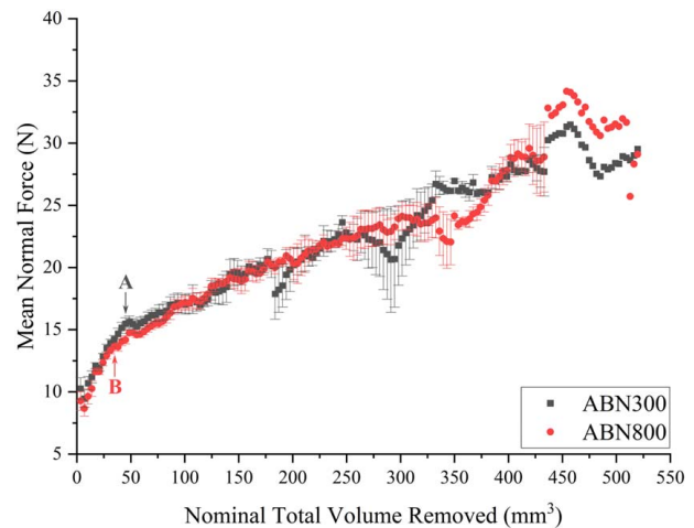
Fig. 4 Evolution of the normal grinding forces during point grinding, including standard errors. Estimated steady-state transition points are marked.
