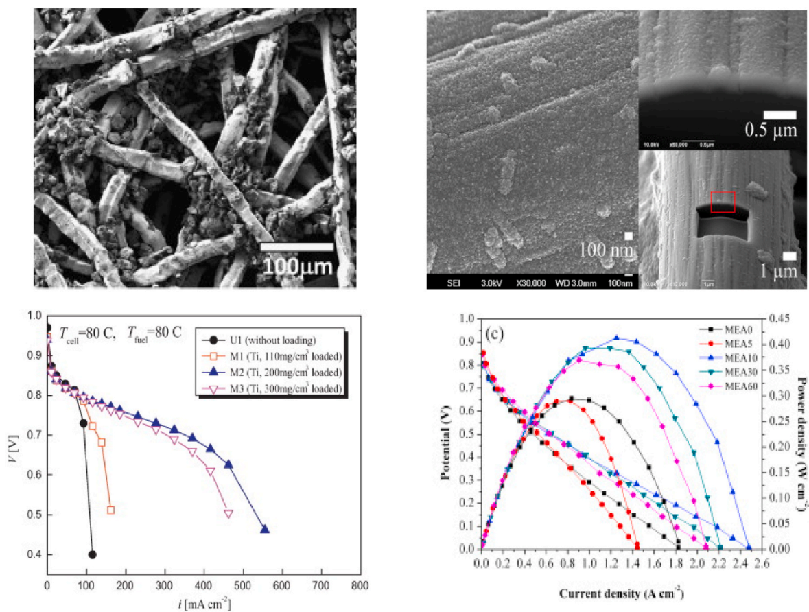
Fig. 19. Titanium coated GDL. (Left) SEM micrograph of the Ti felt substrate surface with Ti powder (300 \text{mg cm}^{-3} ) (top) and polarisation curve of Ti substrate with different Ti loading, 80 ^\circ\text{C} (bottom) (Right) SGL 10BA after 10 min Ti sputtering (top), and the polarisation curve and power density of GDL with varying Ti sputtering time, 65 ^\circ\text{C} (bottom) Reproduced with permission from Elsevier [176].
