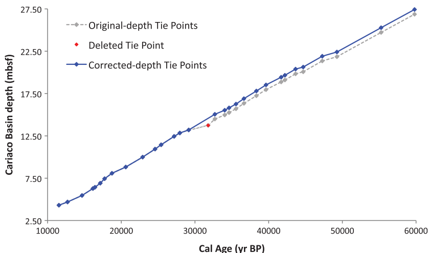
Figure 4 Cariaco-Hulu age-depth models shown over the entire time scale. The revised age-depth curve (blue) is smoother overall and shows fewer abrupt changes than previously (gray).
