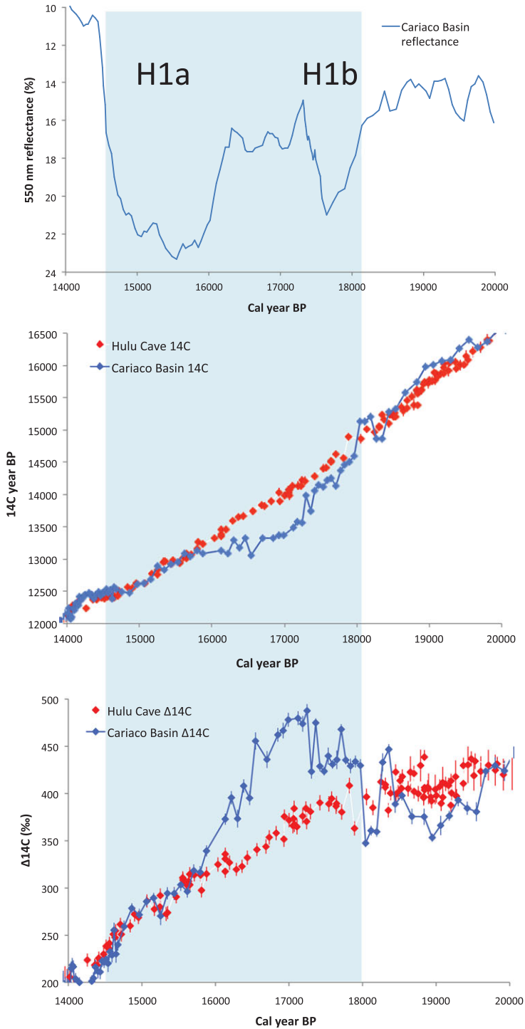
Figure 10 Same as for Figure 9 but focusing on the period surrounding Heinrich Event 1.
