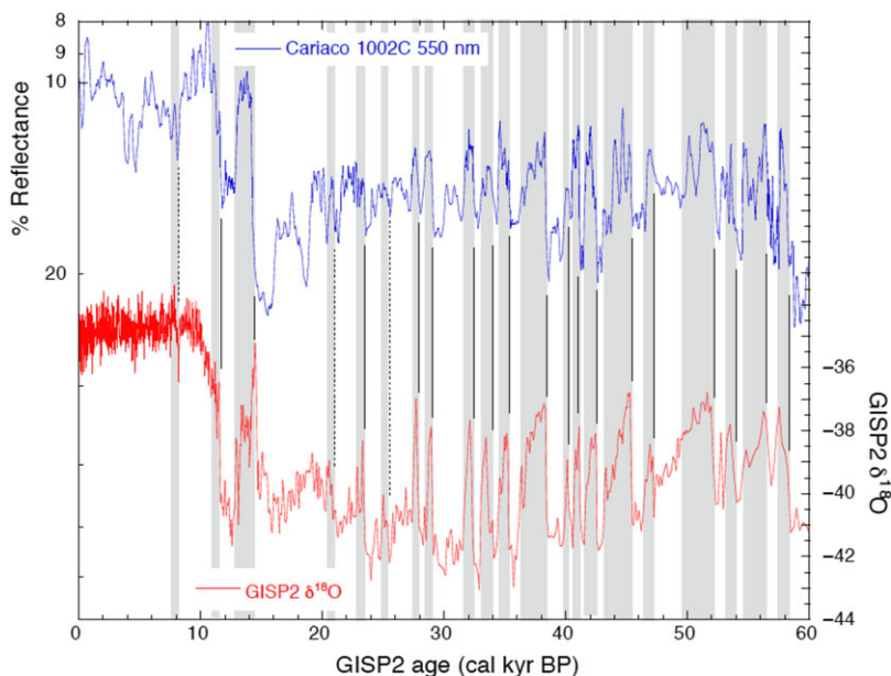
Figure 1 Comparison of paleoclimate records between the Cariaco Basin and Greenland ice cores: (upper) 550 nm reflectance from Cariaco sediments, showing periods of greater windiness (down) and greater rainfall (up). (lower) Oxygen isotopes from the GISP2 ice core, showing periods of increased cooling (down) and warmth (up). These tie points were used in creating the calendar age for the Cariaco Basin ^{14}\text{C} calibration dataset used in IntCal04. Figure adapted from Hughen et al. 2004a, supplementary documentation.
