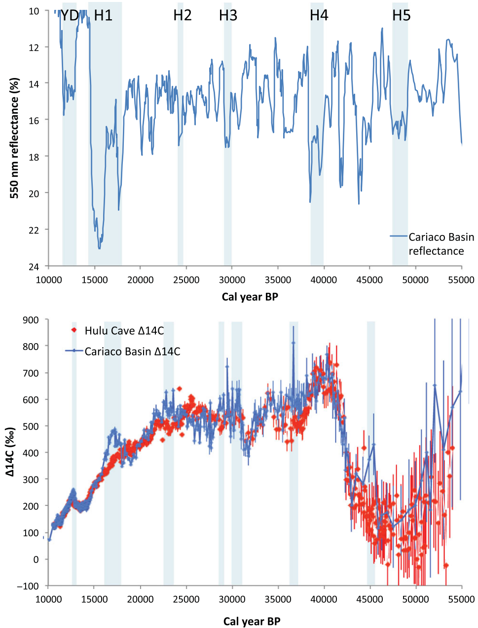
Figure 16 Comparison of timing between Cariaco Basin paleoclimate and ^{14}\text{C} excursions relative to Hulu Cave, shown over entire timescale of the data sets: (upper) 550 nm reflectance from Cariaco sediments, showing periods of greater windiness (down) and greater rainfall (up). The general timing of Heinrich Events in the Cariaco record is shown by light blue bars. (lower) Cariaco Basin (blue) versus Hulu Cave (red) \Delta^{14}\text{C} plots. Periods of reduced Cariaco MRA occur every 6–7 cal kyrs (indicated by light blue bars) but appear distinct from Heinrich Events.
