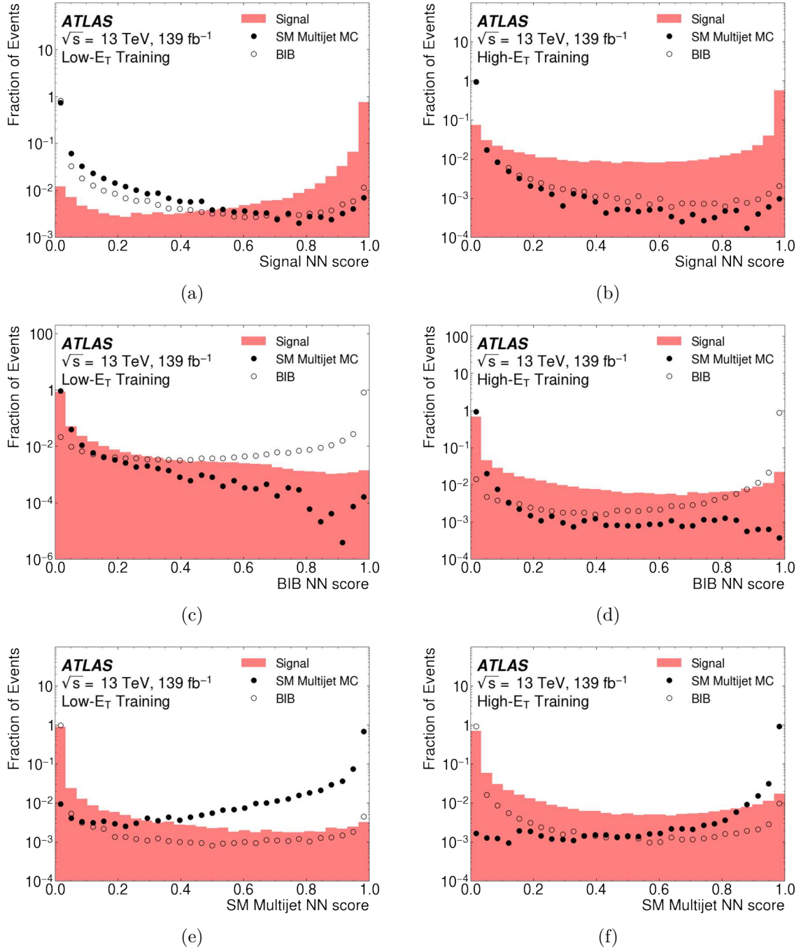
Figure 6. The NN output scores for (a,b) signal, (c,d) BIB and (e,f) SM multijets shown for low- E_T and high- E_T training. The jets used here are part of the validation set, and follow the selection used when choosing jets to train the NN in signal, multijets and BIB.
