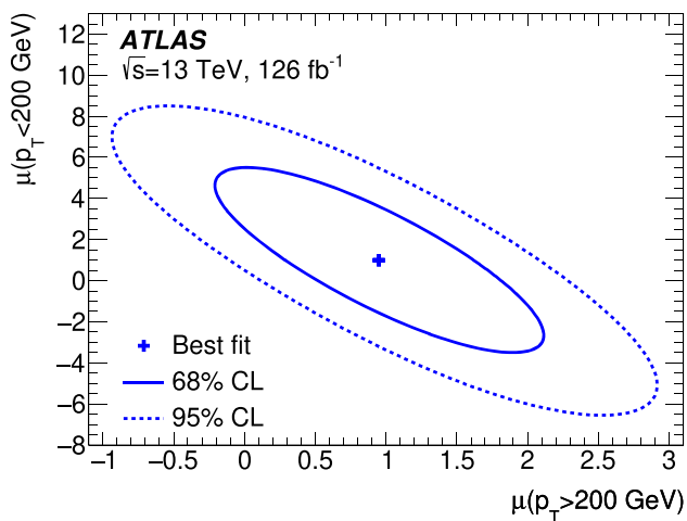
Fig. 7 Likelihood scan as a function of the signal strength for Higgs boson production with true boson p_T > 200 GeV versus the signal strength for Higgs boson production with true boson p_T < 200 GeV. Shown is the best-fit value (blue plus sign), and the 68% (solid blue) and 95% (dashed blue) confidence level (CL) contours
