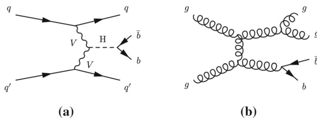
Fig. 1 Feynman diagrams of a the VBF signal process and b gluon splitting as an example background process
