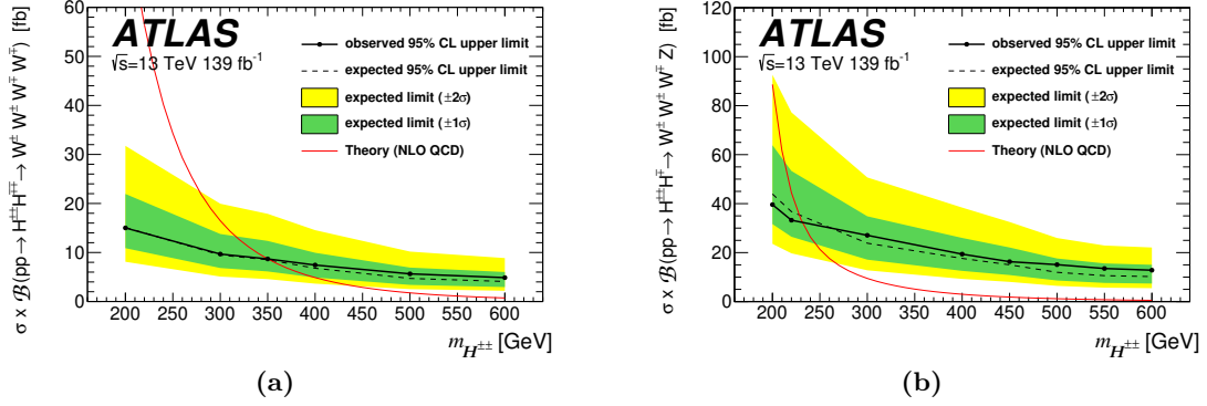
Figure 9. Observed and expected upper limits on the (a) H^{\pm\pm} pair production and (b) H^{\pm\pm} and H^{\pm} associated production cross section times branching fraction at 95% CL obtained from the combination of 2\ell^{\text{sc}} , 3\ell and 4\ell channels. The region above the observed limit is excluded by the measurement. The bands represent the expected exclusion curves within one and two standard deviations. The theoretical prediction [29] including the NLO QCD corrections [52] is also shown.
