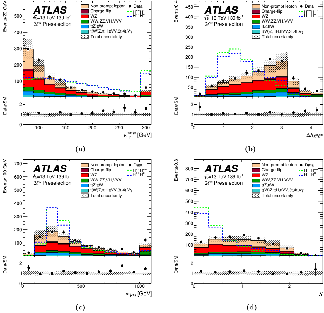
Figure 3. Distribution of selected variables used to define the 2\ell^{\text{sc}} SRs. The events are selected with the preselection requirements listed in table 4. The data (dots) are compared with the expected contributions from the relevant background sources (histograms). The expected signal distributions for m_{H^{\pm\pm}} = 300 GeV are also shown, scaled to the observed number of events. The last bin includes overflows. In each figure the bottom panel shows the ratio of data to the estimated background. The hatched band around unity represents the total uncertainty of the background.
