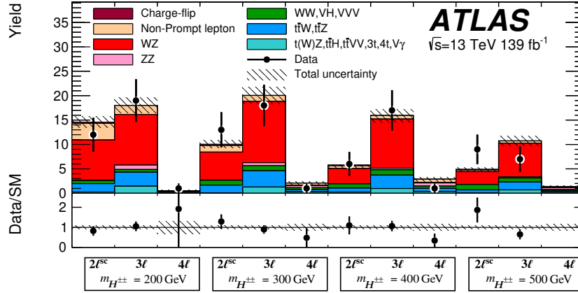
Figure 7. Data event yields compared with the expected contributions from relevant background sources, for the combination of the individual channels of the 2\ell^{sc} , 3\ell and 4\ell SRs. The m_{H^{\pm\pm}} = 220 GeV, 350 GeV and 450 GeV signal hypotheses use the signal regions defined for the m_{H^{\pm\pm}} = 200 GeV, 300 GeV and 400 GeV signal. The m_{H^{\pm\pm}} = 550 GeV and m_{H^{\pm\pm}} = 600 GeV signal hypotheses use the signal regions defined for the m_{H^{\pm\pm}} = 500 GeV signal. The total uncertainties in the expected event yields are shown as the hatched bands.
