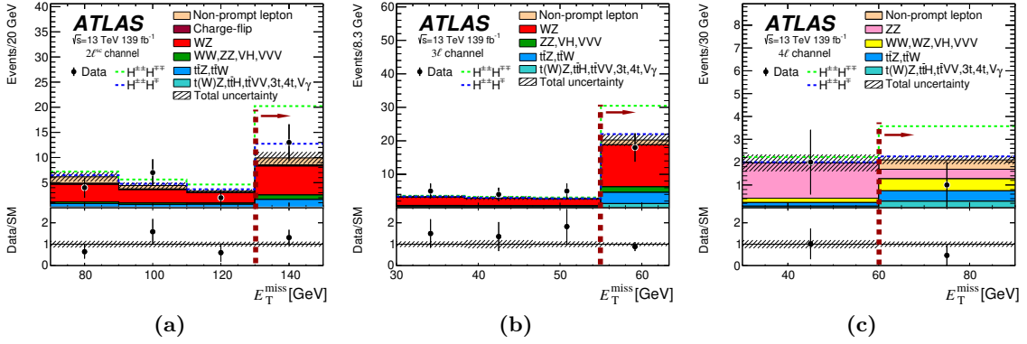
Figure 8. The E_T^{\text{miss}} distribution for the SRs of the m_{H^{\pm\pm}} = 300 GeV signal mass hypothesis, where the selection requirement on E_T^{\text{miss}} has been removed. The distribution is shown for the combination of the individual channels of the (a) 2\ell^{\text{sc}} , (b) 3\ell and (c) 4\ell SRs. The total uncertainties in the expected event yields are shown as hashed bands. The last bin, isolated by a vertical red dashed line, is inclusive and corresponds to the SR. The expected signal distributions corresponding to the m_{H^{\pm\pm}} = 300 GeV are also shown (stack histogram, on top of the background). In each figure the bottom panel shows the ratio of data to the estimated background. The hatched band around unity represents the total uncertainty of the background.
