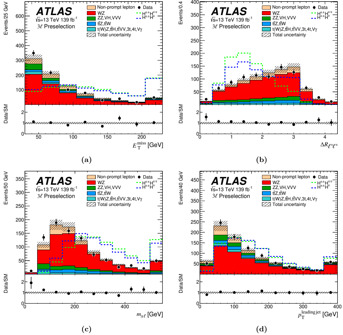
Figure 4. Distribution of selected variables used to define the 3\ell SRs. The events are selected with the preselection requirements listed in table 4. The data (dots) are compared with the expected contributions from the relevant background sources (histograms). The expected signal distributions for m_{H^{\pm\pm}} = 300 GeV are also shown, scaled to the observed number of events. The last bin includes overflows. In each figure the bottom panel shows the ratio of data to the estimated background. The hatched band around unity represents the total uncertainty of the background.
