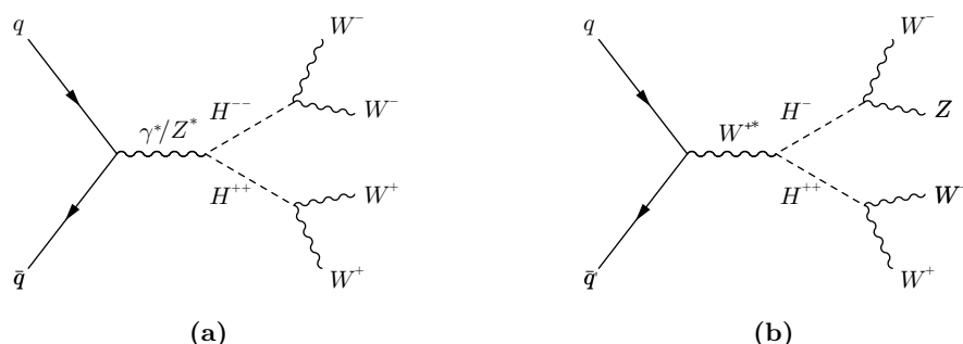
Figure 1. Feynman diagrams illustrating production and subsequent decay of the H^{\pm\pm} and H^{\pm} bosons: (a) H^{\pm\pm} pair production and (b) H^{\pm\pm} and H^{\pm} associated production.
