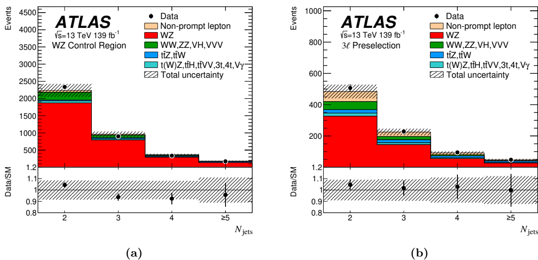
Figure 2. Distribution of the jet multiplicity in the (a) WZ control region and in the (b) 3\ell preselection region. The data (dots) are compared with the estimated contributions from the background sources (histograms). The normalisation factor is applied to the WZ MC contribution. The last bin includes overflows. In each figure the bottom panel shows the ratio of data to the estimated background. The hatched band around unity represents the total uncertainty of the background.
