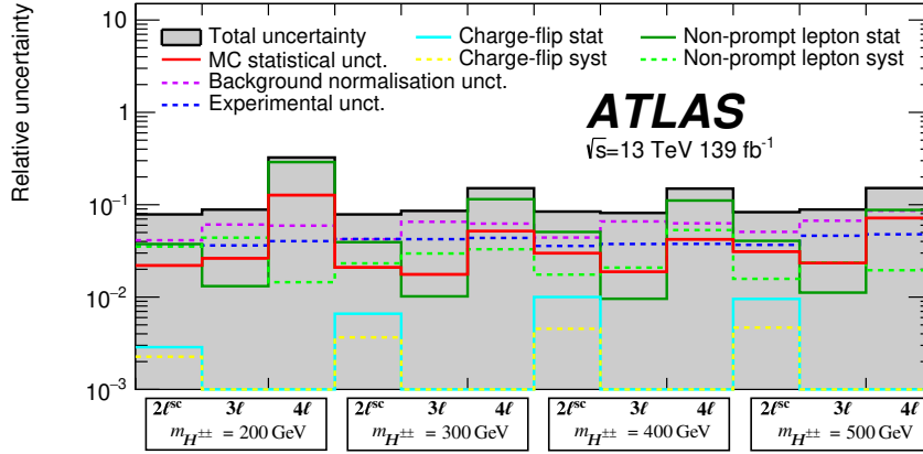
Figure 6. Contributions from different categories of uncertainties relative to the expected background yields in the defined SRs. The uncertainties are shown for the combination of the individual channels of the 2\ell^{sc} , 3\ell and 4\ell SRs. The m_{H^{\pm\pm}} = 220 GeV, 350 GeV and 450 GeV signal hypotheses use the signal regions defined for the m_{H^{\pm\pm}} = 200 GeV, 300 GeV and 400 GeV signal. The m_{H^{\pm\pm}} = 550 GeV and m_{H^{\pm\pm}} = 600 GeV signal hypotheses use the signal regions defined for the m_{H^{\pm\pm}} = 500 GeV signal. The SRs are indicated along the horizontal axis.
