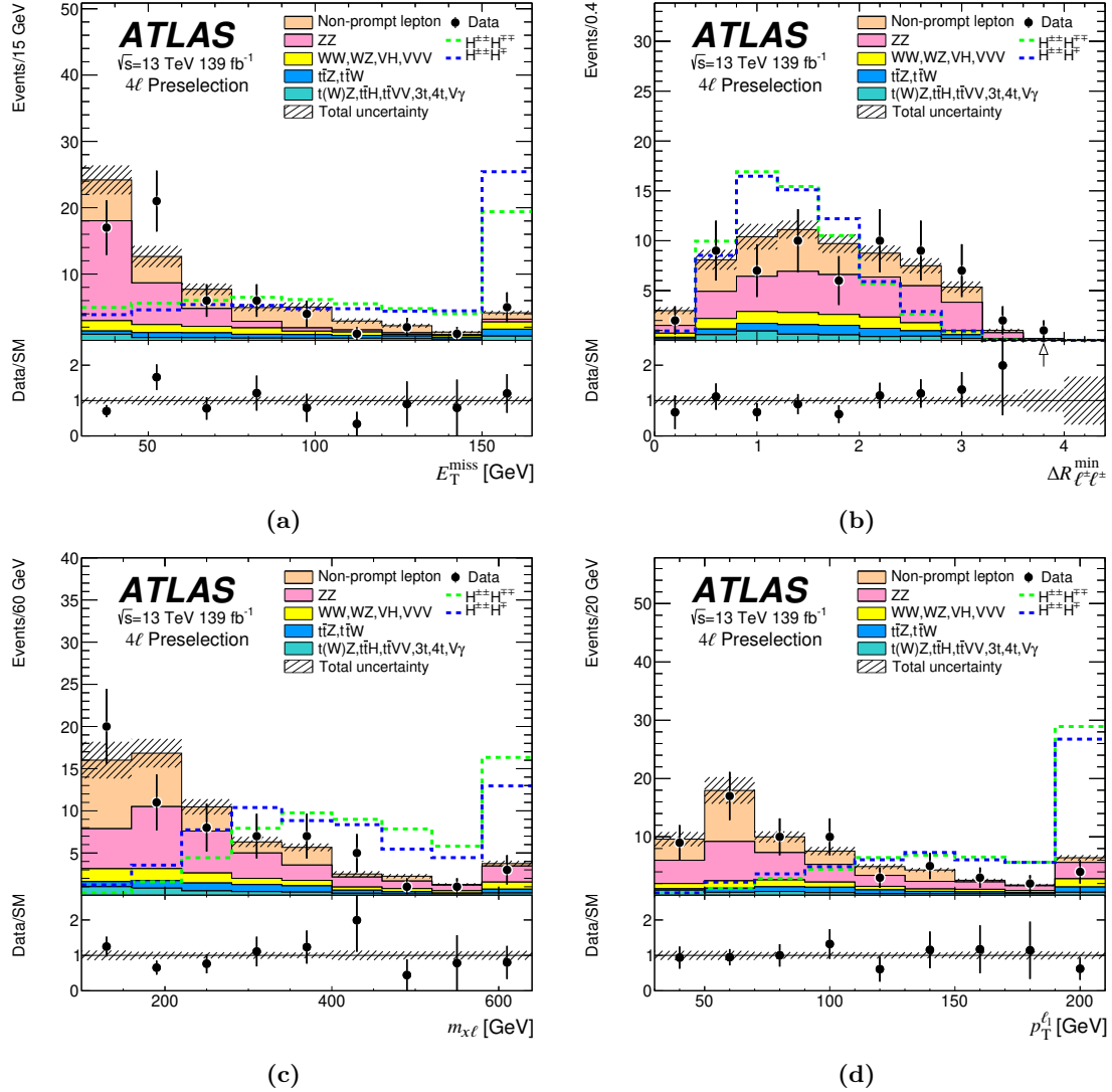
Figure 5. Distribution of selected variables used to define the 4\ell SRs. The events are selected with the preselection requirements listed in table 4. The data (dots) are compared with the expected contributions from the relevant background sources (histograms). The expected signal distributions for m_{H^{\pm\pm}} = 300 GeV are also shown, scaled to the observed number of events. The last bin includes overflows. In each figure the bottom panel shows the ratio of data to the estimated background. The hatched band around unity represents the total uncertainty of the background.
