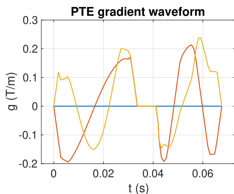
FIGURE 2 The gradient waveform of the planar tensor encoding
