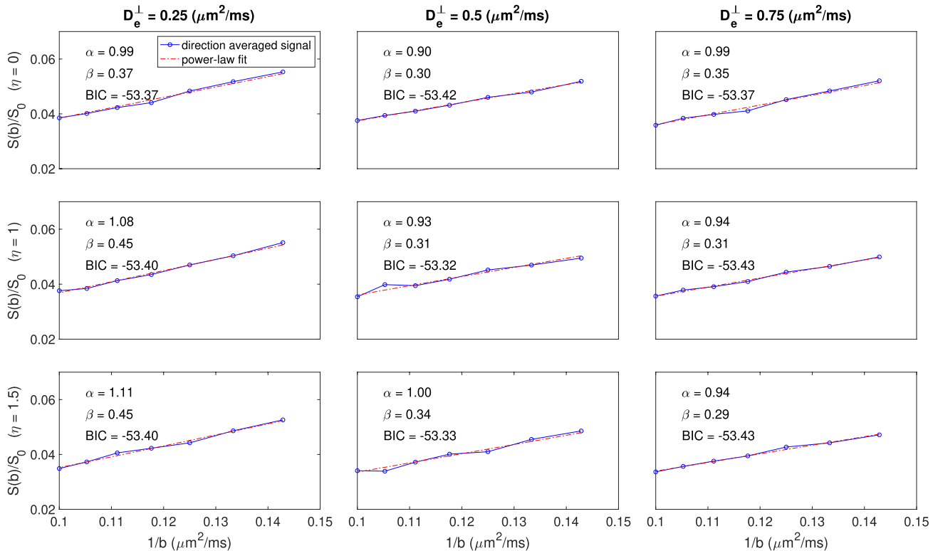
FIGURE 4 Simulated direction-averaged PTE signal for 7000 < b < 10000 \text{ s/mm}^2 and the results of the power-law fit
