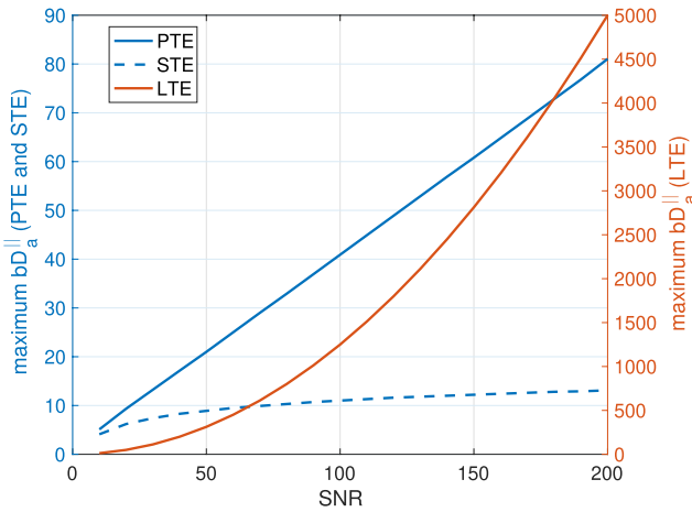
FIGURE 3 Maximum bD_a^{\parallel} vs SNR. The Maximum bD_a^{\parallel} value is proportional to the square of SNR, ( bD_a^{\parallel} \sim SNR^2 ) for LTE, where this relationship is linear for PTE ( bD_a^{\parallel} \sim SNR ) and it is logarithmic for STE ( bD_a^{\parallel} \sim \ln(SNR) )
