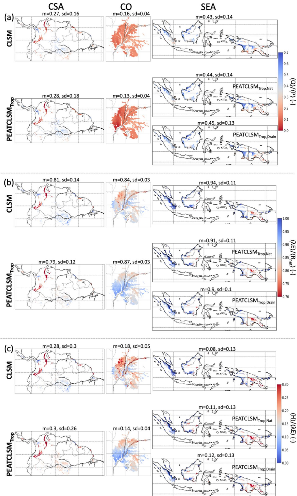
Figure 9. The 20-year (1 January 2000 through 31 December 2019) mean (a) runoff efficiency \langle(Q)/(P)\rangle , (b) evapotranspiration efficiency \langle(\lambda E)/(R_{net})\rangle , and (c) Bowen ratio \langle(H)/(\lambda E)\rangle for CLSM and PEATCLSM Trop simulations over the three study regions: (left) Central and South America, (middle) the Congo Basin, (right) Southeast Asia. For Southeast Asia, both PEATCLSM Trop,Nat and PEATCLSM Trop,Drain are shown. The titles provide the spatial mean (m) and standard deviation (sd). Note the inverse color bar in (c).
