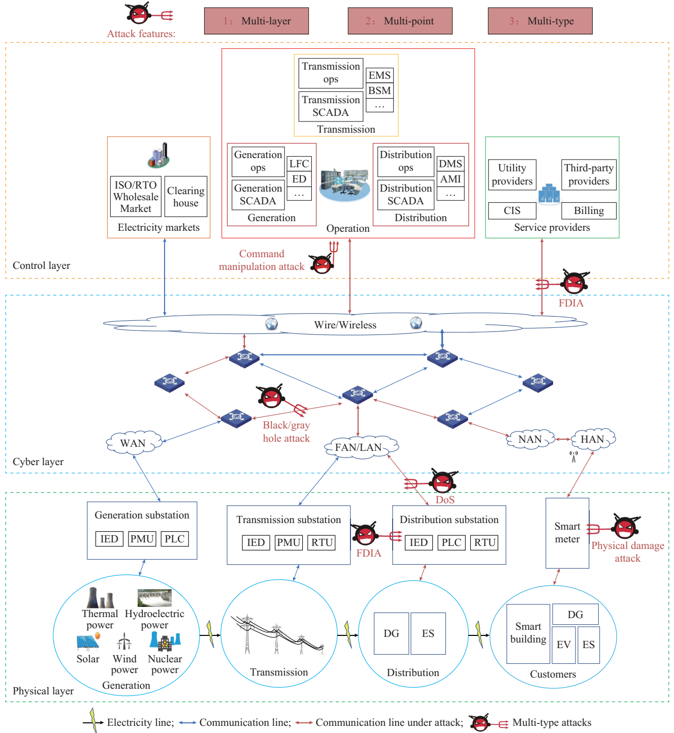
Fig. 4. Framework of CPPSs under multi-type attacks.
