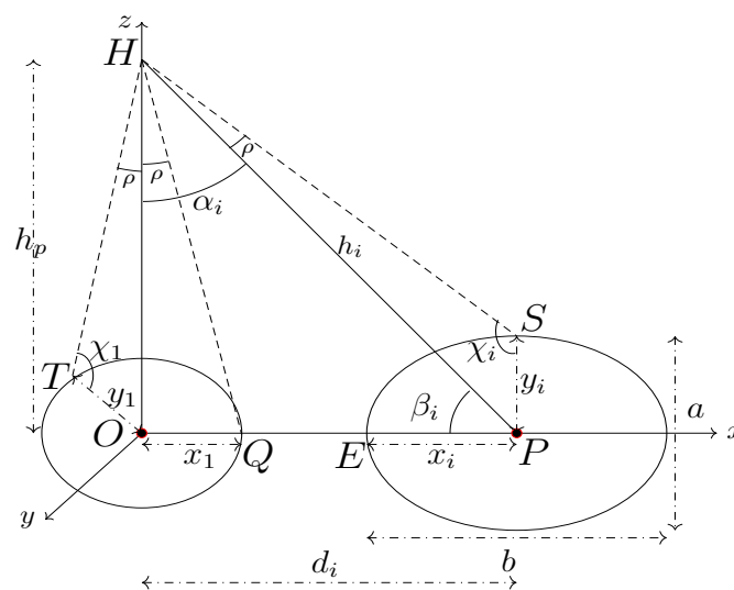
Figure 4. HAP elliptical cell geometry (semi-minor axis)
