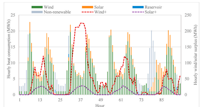
Fig. 3. The supply mix and wind/solar surplus 1–4 Jul 2018 – Group A.
