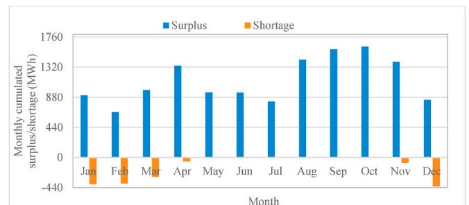
Fig. 8. Monthly accumulated hourly surplus (from wind/solar/sewer heat) and monthly accumulated hourly shortage.
