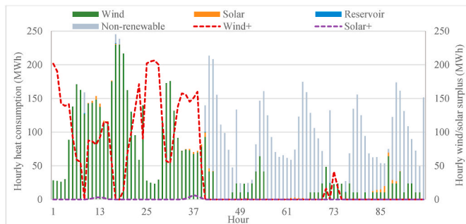
Fig. 2. The supply mix and wind/solar surplus 1–4 Feb 2018 – Group A.
