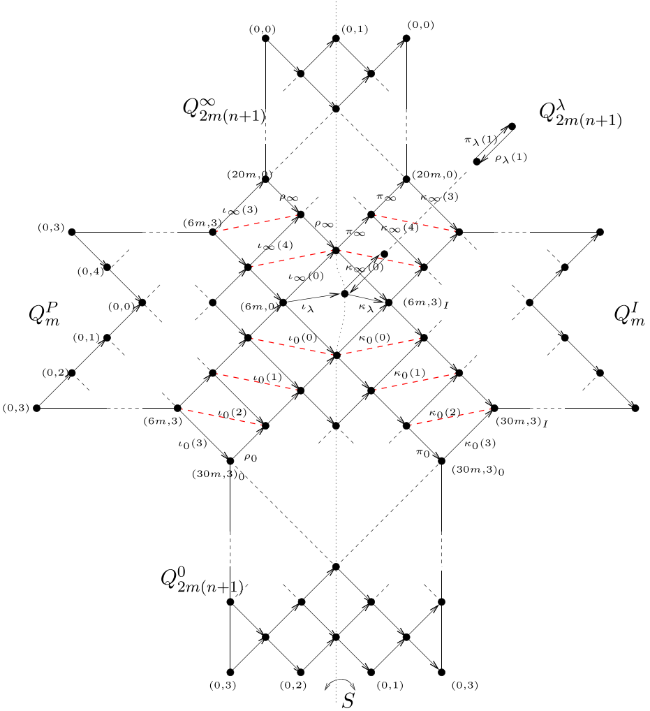
Fig. 2 Q_m for g = 3, n = 4
