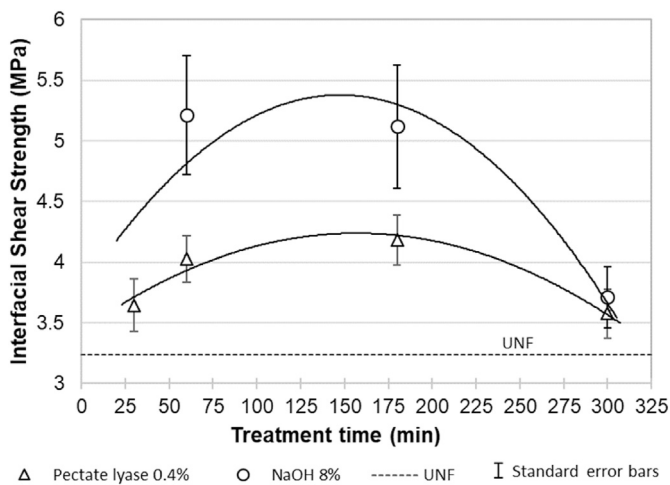
Fig. 10. Effect of treatment time on interfacial shear strength for agave tequilana fibres treated with 8% NaOH and 0.4% Pectate Lyase.
