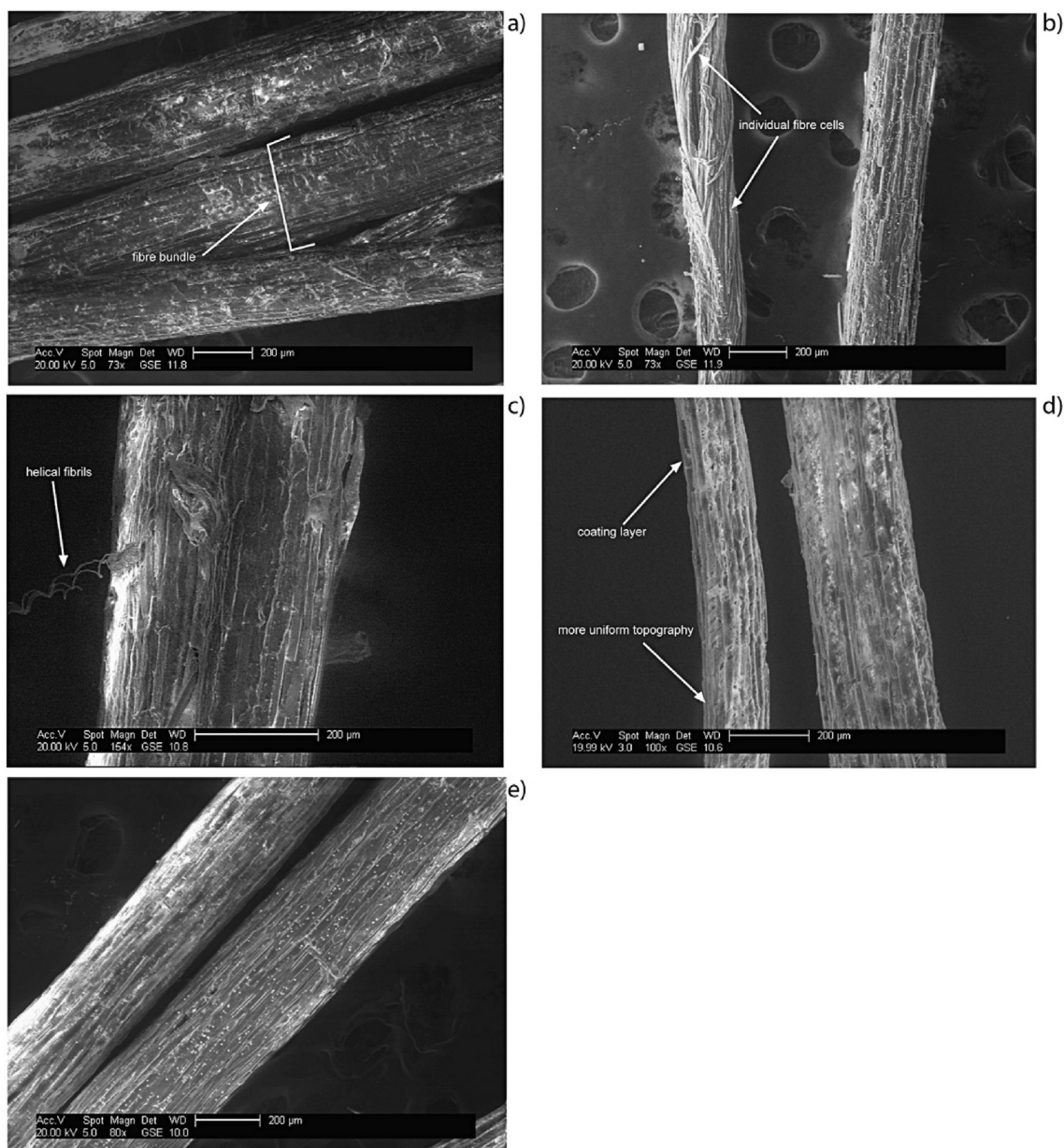
Fig. 4. ESEM of untreated and treated agave tequilana fibres: a) UNF presenting a closely packed fibre bundle; b) AKF (NaOH 8% - 180 min) showing loose fibre bundles; c) ENF (pectate lyase 4% - 60 min) showing partially loose fibre bundles; d) ACF ((CH 3 CO) 2 O 50% - 120 min) showing a more uniform and coated fibre bundle; e) SIF (APTES 10% - 60 min) presenting a uniform fibre bundle.
