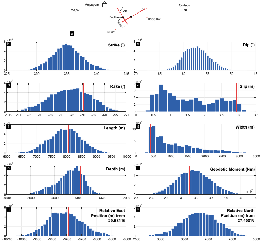
Fig. 2 a Schematic diagram of the relative location of the two possible fault plane solutions for the Acipayam earthquake. In one solution, the fault plane dips steeply to the ENE, in the other it dips more shallowly to the WSW (solid red lines). The up-dip projections of the fault planes to the surface are denoted by dashed red lines. As the modelled slip increases, the width of these fault lines collapse to approximately the same point in the modelling due to trade-offs between these two parameters for buried sources. The relative locations of the seismological solutions are indicated by red stars. b–k Modelling results for fault parameters (location, size, orientation and slip) and parameter uncertainties (posterior probability distributions) through Bayesian analysis using GBIS (Bagnardi and Hooper 2018) for the eastward dipping fault plane solution based upon the data in Fig. 1. The best fit fault model for each parameter is shown by the red line, with the histogram of the distributions of solutions shown in blue for 800,000 model iterations (Table 2 has the best fit model and range of solutions). The fault plane location (upper midpoint of slip area) is given relative to a reference point 29.531° E, 37.408° N which is the USGS epicentre
