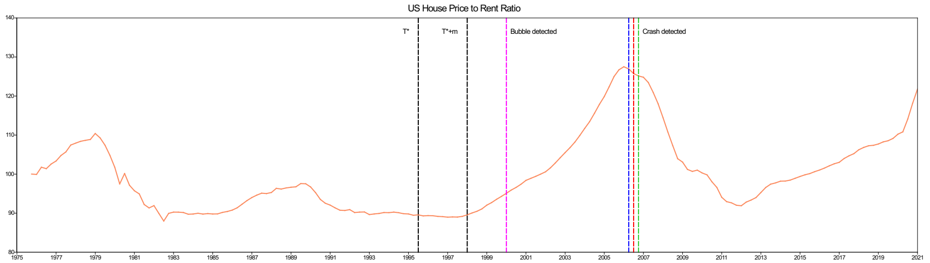
Figure 8: US house price to rent ratio and S_{MIN}(m, n) test statistics, 1975-2021
