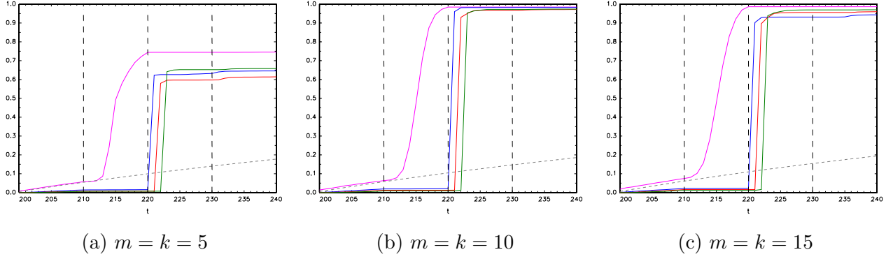
Figure 2: Rejection frequencies of A_{MAX}(k) and S_{MIN}(m, n) , and histograms of S_{MIN}(m, n) detection dates: \lfloor \tau_1 T \rfloor = 210 , \lfloor \tau_2 T \rfloor = 220 , \lfloor \tau_3 T \rfloor = 230 , \delta_1 = 0.03 and \delta_2 = 0.015
