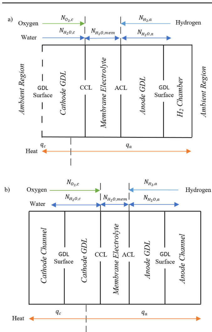
Fig. 1. Schematic representations of the modelled: (a) air-breathing and (b) conventional PEFCs. Note that the symbol 'N' stands for molar flux, 'q' for heat flux, 'CCL' for cathode catalyst layer and 'ACL' for anode catalyst layer, the subscript 'a' for anode and the subscript 'c' for cathode.
