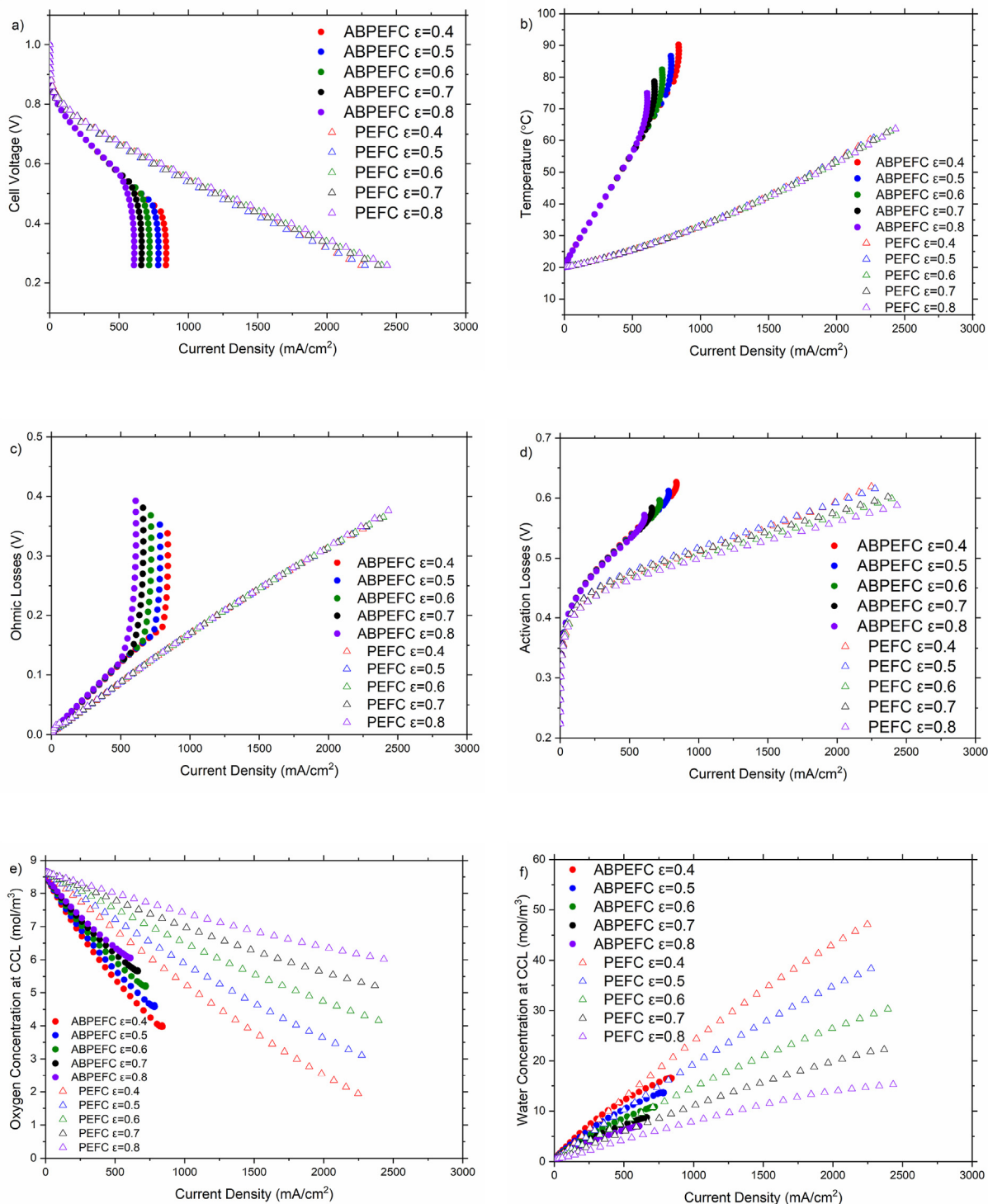
Fig. 3. The outputs of the modelled air-breathing and conventional PEFCs at 20 °C and 40% relative humidity and variable cathode GDL porosity: (a) cell voltage, (b) cell temperature, (c) ohmic losses, (d) activation losses, (e) oxygen concentration at the cathode catalyst layer and (f) water concentration at the cathode catalyst layer as a function of current density.
