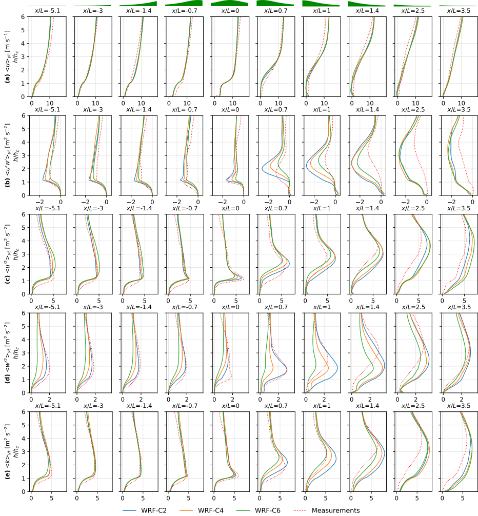
Fig. 5 Vertical profiles of time and y-direction averaged (from the top to bottom panels) stream-wise velocity \langle u \rangle_{yT} , vertical momentum flux per unit mass \langle u'w' \rangle_{yT} , stream-wise velocity variance \langle u'^2 \rangle_{yT} , vertical velocity variance \langle w'^2 \rangle_{yT} and turbulence kinetic energy per unit mass \langle k \rangle_{yT} for WRF-C, compared with the wind-tunnel measurements over the ‘Furry Hill’ from Finnigan and Brunet (1995) (see text for details). A graphical representation of the slope in the terrain present around each profile is displayed at the top of the figure
