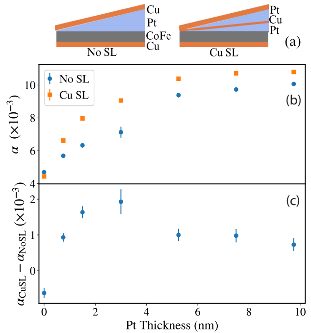
FIG. 6. (a) Schematic of systems with and without a Cu SL within the Pt. (b) Measured damping parameter from the FMR linewidth for Cu(2 nm)/CoFe(7 nm)/Pt[ t (nm)] and Cu(2 nm)/CoFe(7 nm)/Pt[ t/2 (nm)]/Cu(5 nm)/Pt[ t/2 (nm)] systems. (c) Difference in the damping parameter between the two systems.
