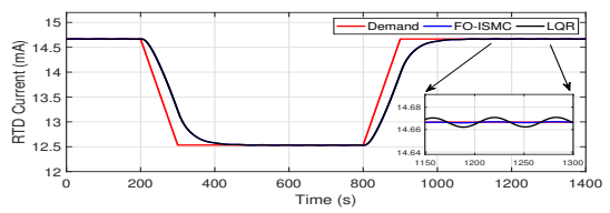
Fig. 13. RTD current.
