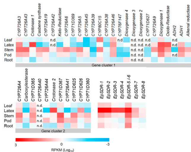
Fig. 2. Expression levels of candidate genes from two casbene-derived diterpenoid gene clusters and a non-clustered gene family of SDRs expressed predominantly in E. pepplus latex. Genes from the two E. pepplus casbene-derived diterpenoid gene clusters are ordered according to relative genomic location. RPKM, reads per kilobase of transcript, per million mapped reads; n.d., no reads detected.
