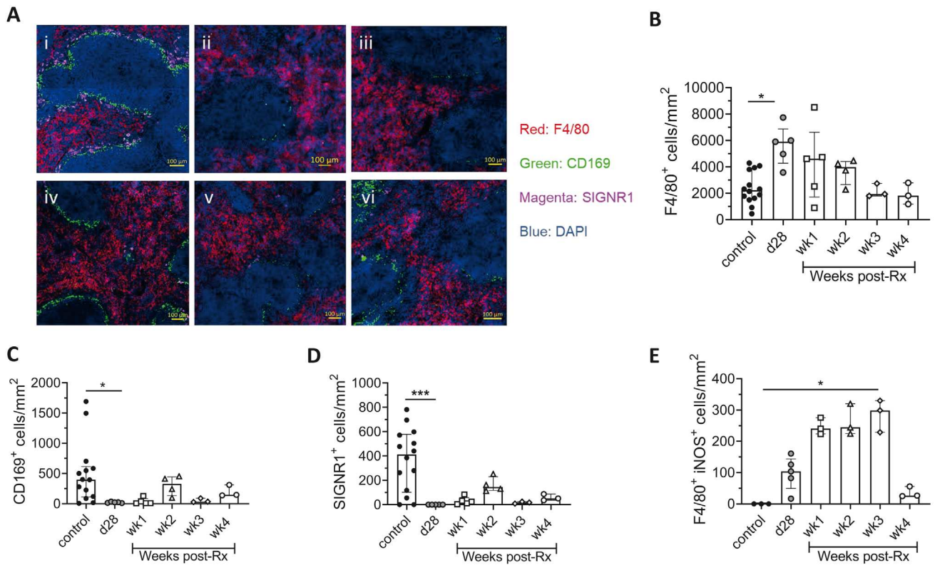
Figure 3. Restoration of splenic microarchitecture in drug-treated L. donovani infected mice. A Spleen sections of (i) uninfected control, (ii) d28, (iii) wk1, (iv) wk2, (v) wk3, (vi) wk4. post-Rx mice were stained with macrophage markers, DAPI (Blue); nuclei, F4/80 (Red); RP macrophages, CD169 (Green) and SIGNR1 (Magenta) for MMM and MZM respectively, scale bar; 100 \mu m. B-D The number of F4/80 + RP macrophages ( B ), CD169 + MMM ( C ) and SIGNR1 + MZM ( D ) after treatment with AmBisome® was determined by segmentation analysis. Data are amalgamated from two independent experiments with n=14 uninfected control (Expt. 1 and 2), n=5 d28 infected (Expt. 2) and n=3-5 treated mice per time-point post-Rx (Expt. 1). Data shown as median with quartiles and were analysed using non-parametric Kruskal-Wallis test with Dunn's post-hoc test, *, p < 0.05; ***, p < 0.001. E The number of iNOS + F4/80 + cells per unit area was determined by segmentation analysis. Data are representative of n=3 uninfected control mice, n=5 d28 infected mice and n=3 treated mice at weeks 1-4 post-Rx, as above. Data shown as median with quartiles and were analysed using non-parametric Kruskal-Wallis test with Dunn's post-hoc test, *, p < 0.05.
